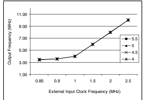
Figure 46. PLLx8 Output vs CLKIN frequency
