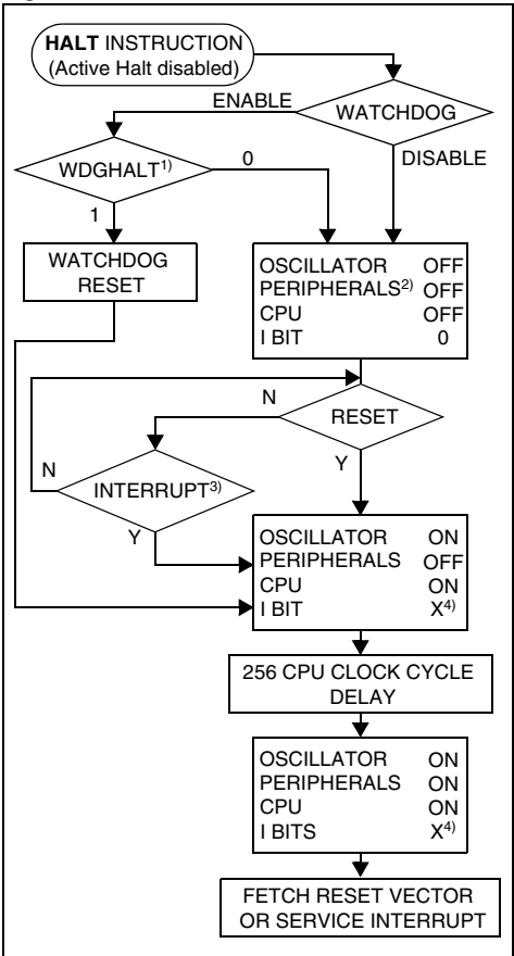
Figure 22. HALT Mode Flowchart
