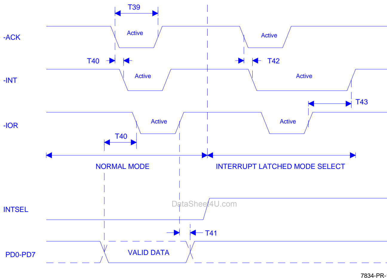
Interrupt timing
