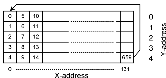
Figure 9 Addressing Mode: Vertical (V=1)
