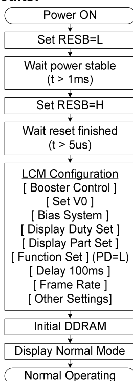
Figure 20 Initial flow with built-in Power Supply Circuits
