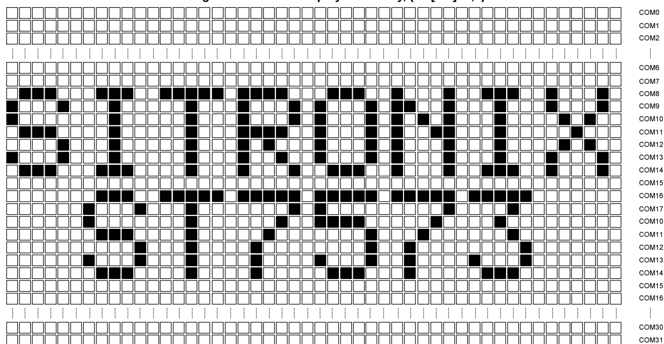
Figure 17 Partial Display: 1/17 Duty, (DP[1:0]=0,1)
