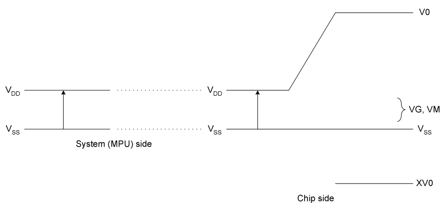
Figure 22 Voltage Range
