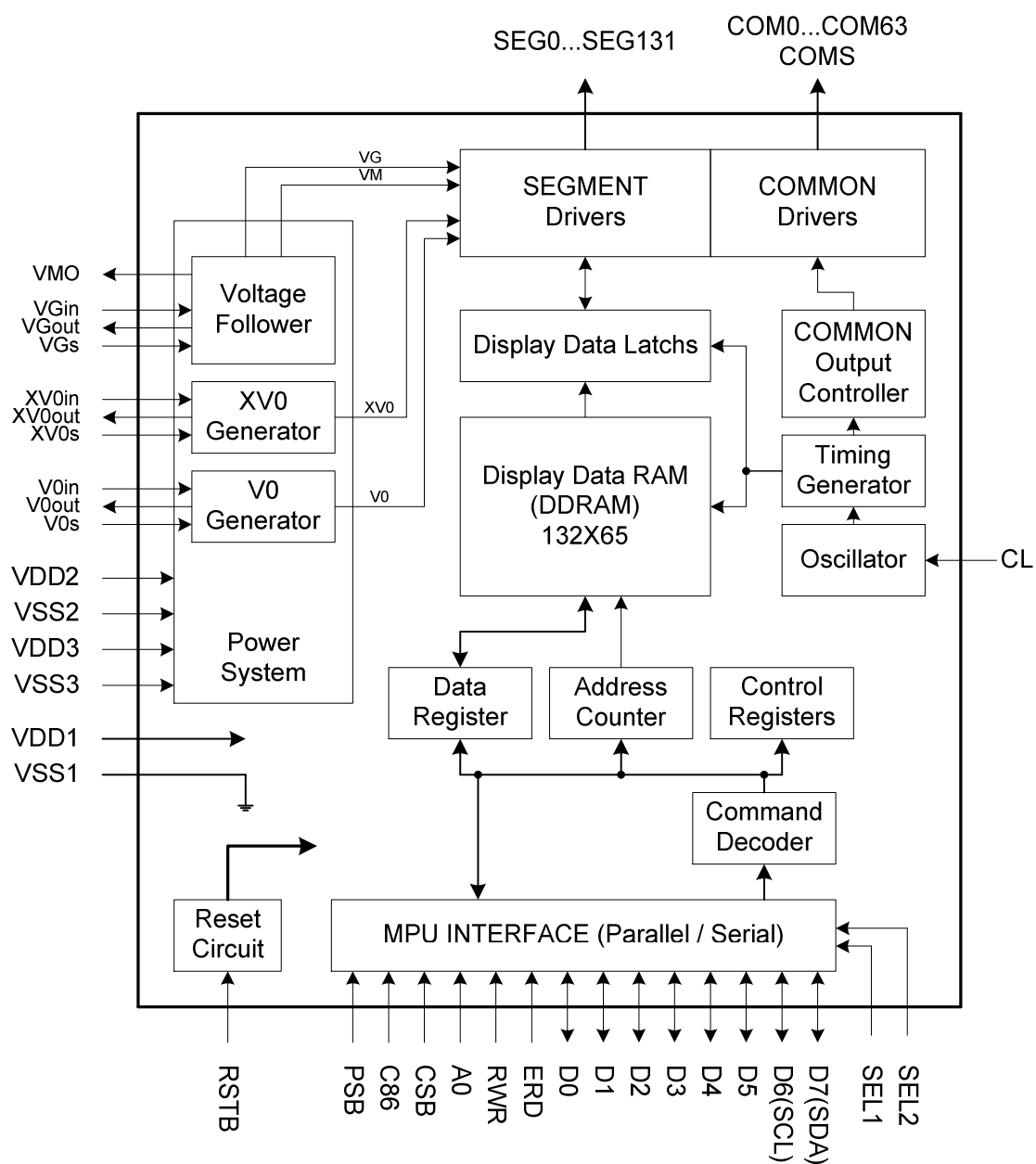
Fig 3. Block Diagram
