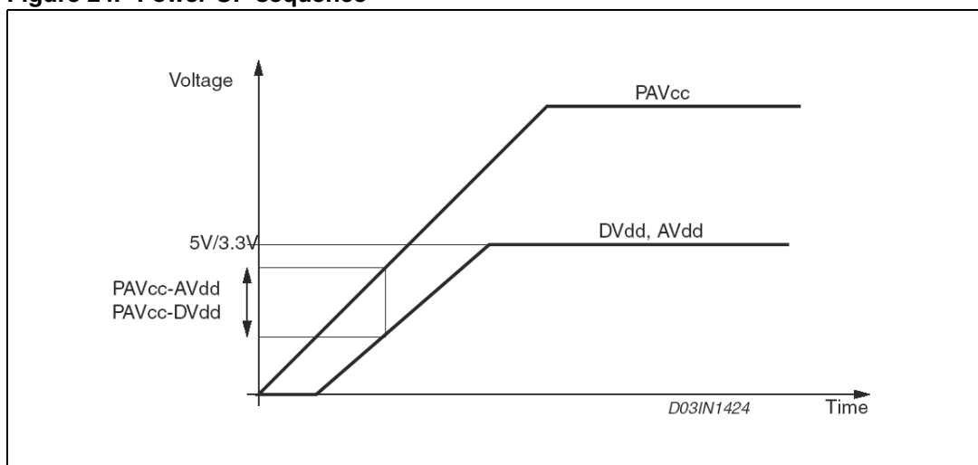
Figure 24. Power-UP sequence
