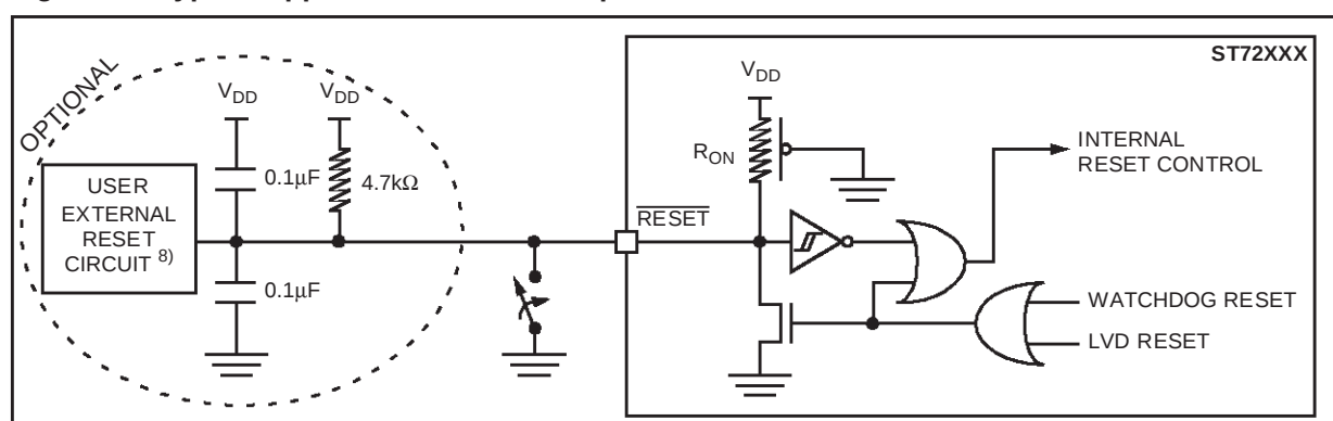
Figure 90. Typical Application with RESET pin 8)
