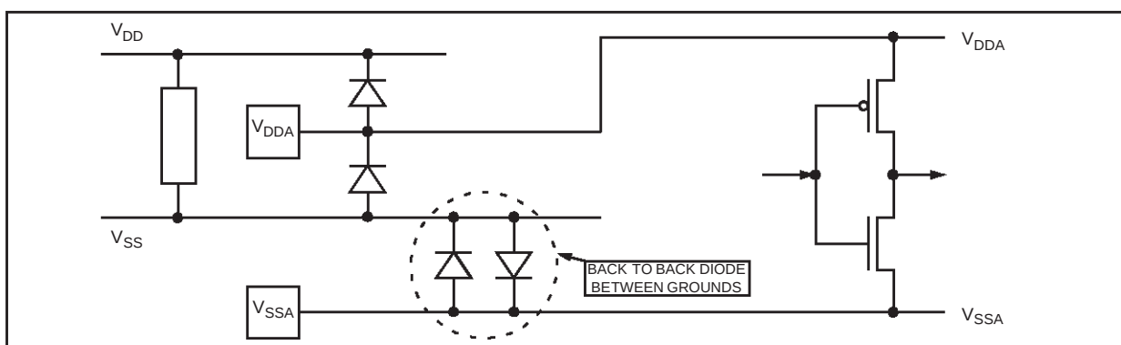
Figure 81. Multisupply Configuration
