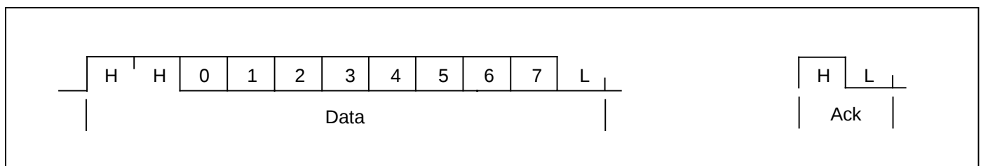
Figure 12.1 OS-Link data and acknowledge formats
