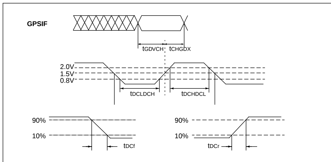
Figure 19.5 ClockIn timings
