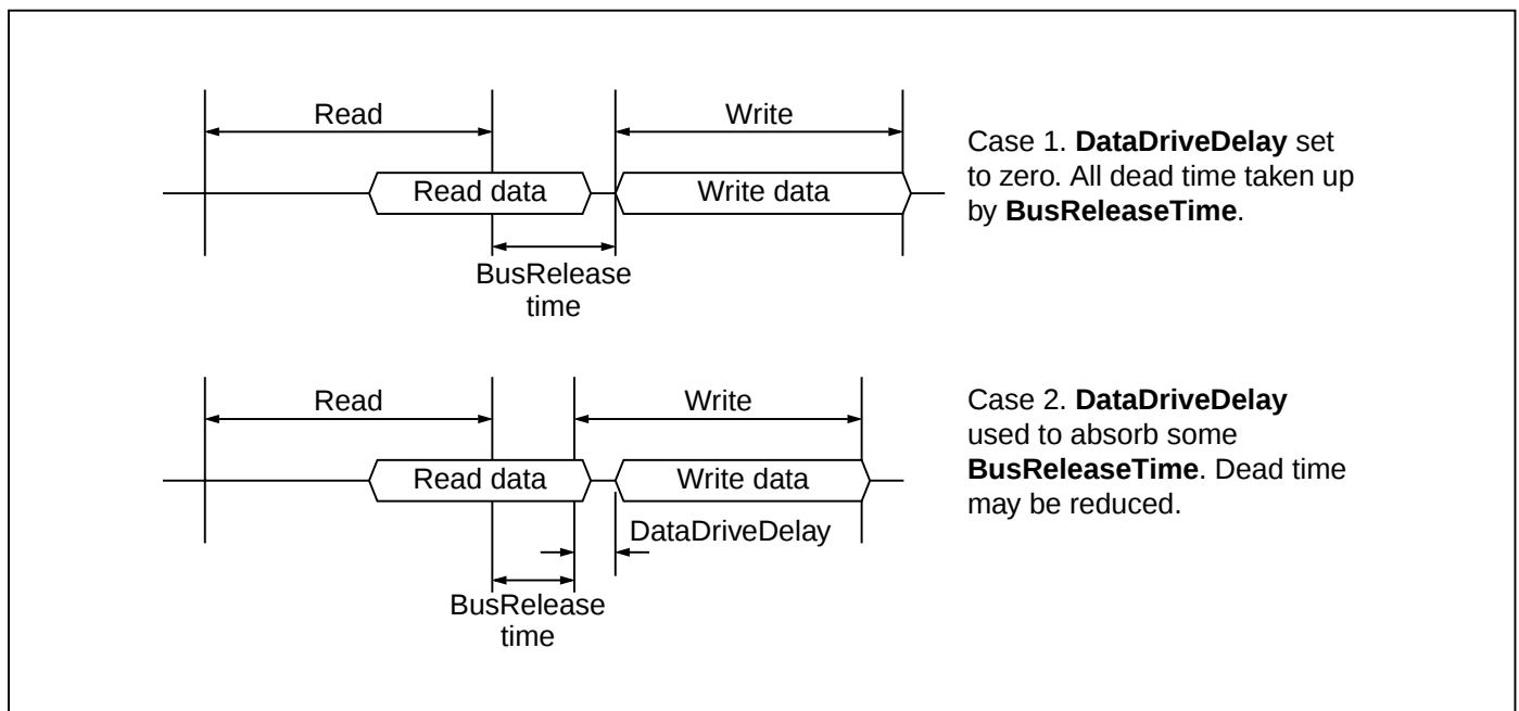
Figure 9.4 Use of DataDriveDelay parameter
