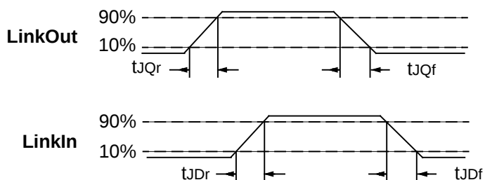
Figure 19.2 Link timings
