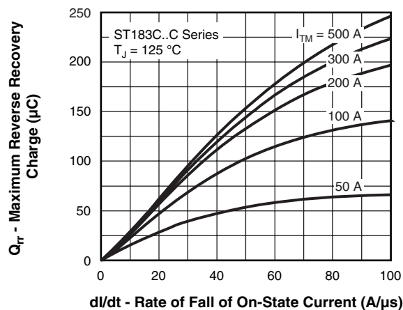
Fig. 11 - Reverse Recovered Charge Characteristics
