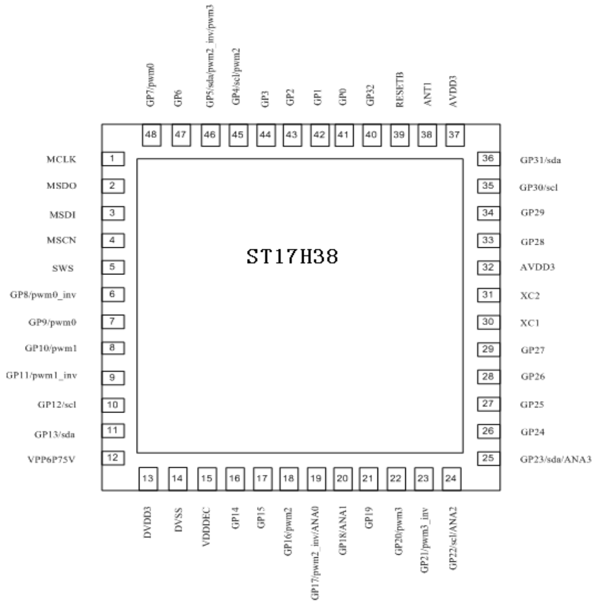
Figure 1- 6 Pin assignment for the ST17H38ET48
