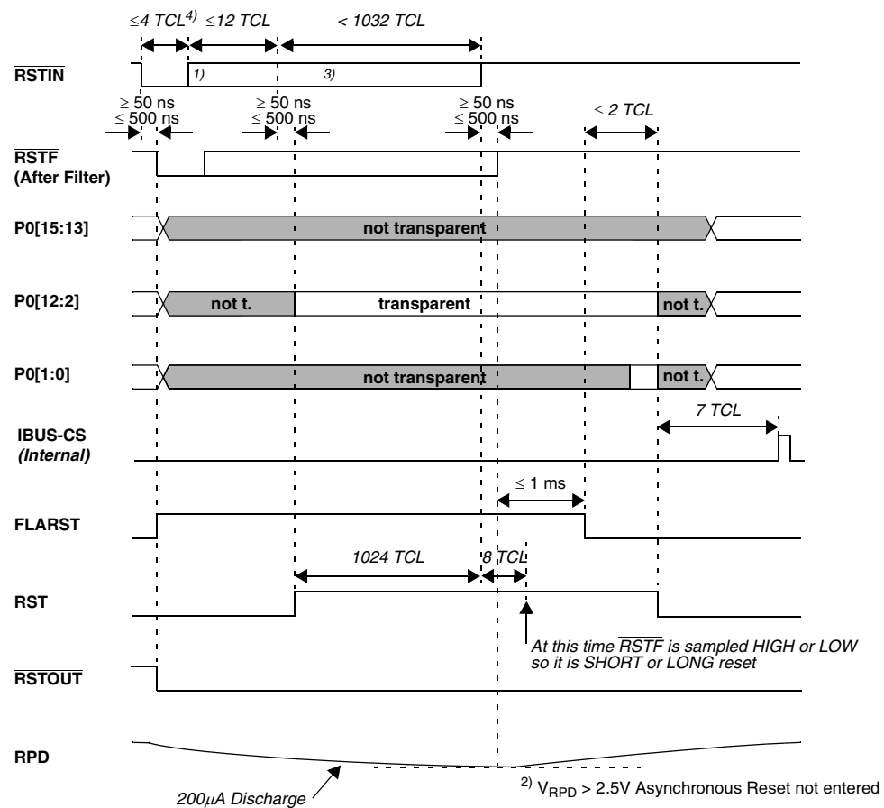
Figure 21. Synchronous short / long hardware RESET ( \overline{EA} = 1 )
