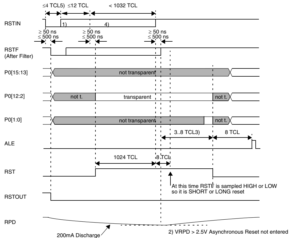
Figure 22. Synchronous short / long hardware RESET ( \overline{\text{EA}} = 0 )
