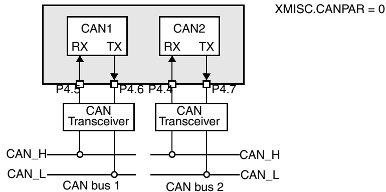
Figure 15. Connection to two different CAN buses (e.g. for gateway application)
