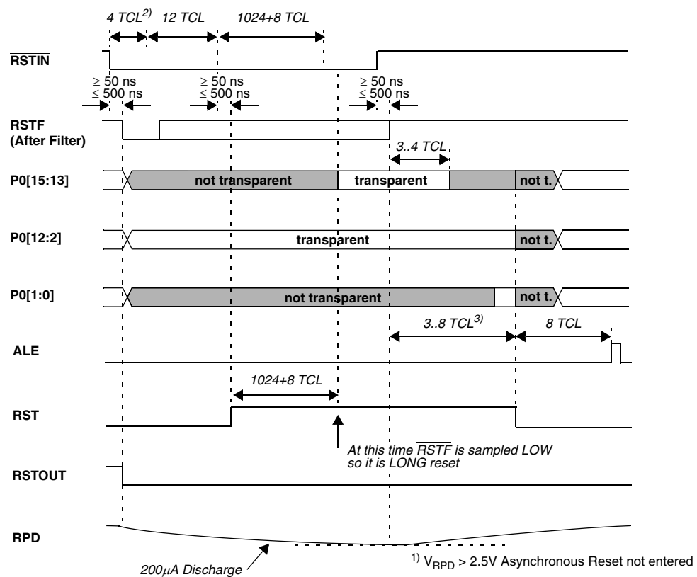
Figure 24. Synchronous long hardware RESET ( \overline{EA} = 0 )
