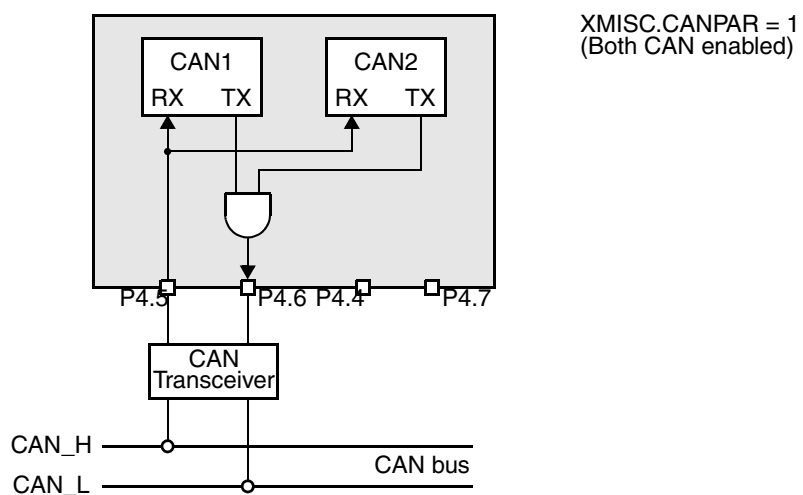
Figure 16. Connection to one CAN bus with internal Parallel Mode enabled
