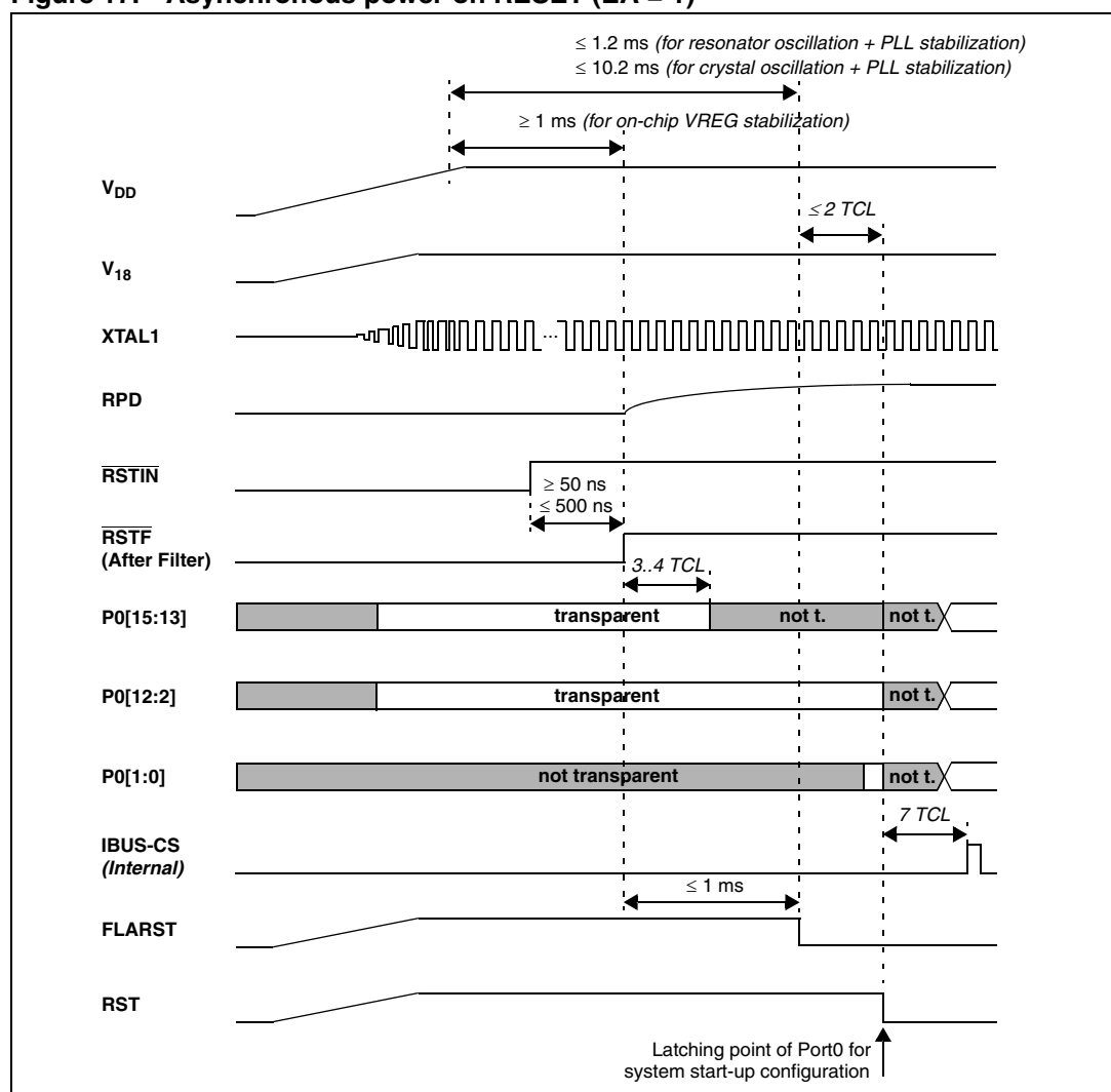
Figure 17. Asynchronous power-on RESET ( \overline{\text{EA}} = 1 )
