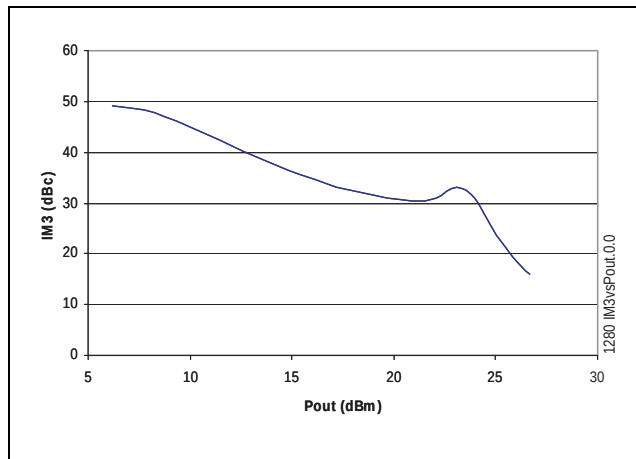
FIGURE 8: IM3 vs P_{OUT}
