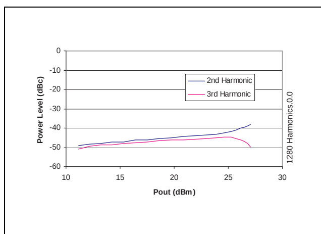
FIGURE 9: HARMONICS
