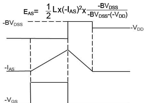
Fig.8 E_{AS} Waveform
