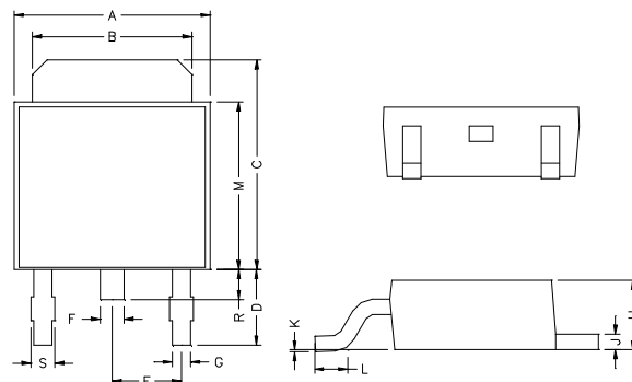
TO-252
