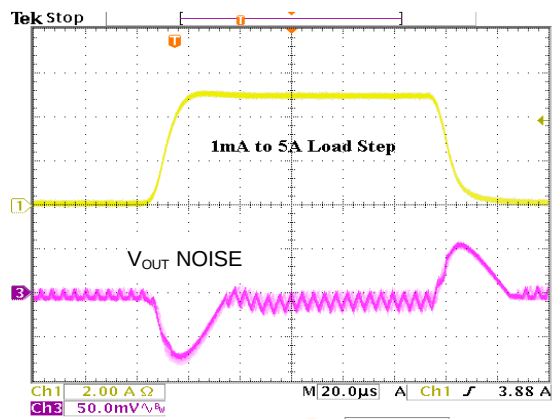
Fig. 5 Transient Response
