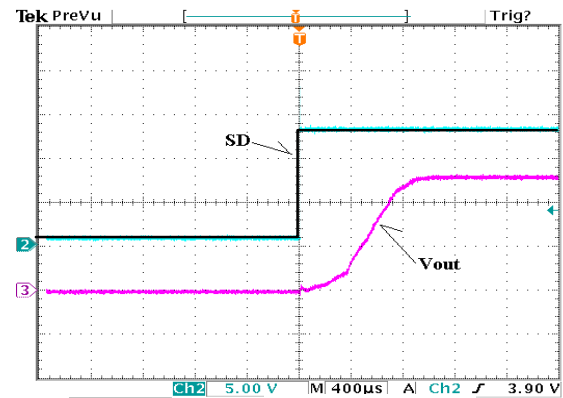
Fig. 4 Output Clamped by Built-In Soft Start
