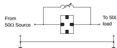
Typical Test Circuit
