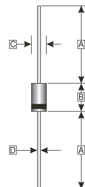
DO-41
