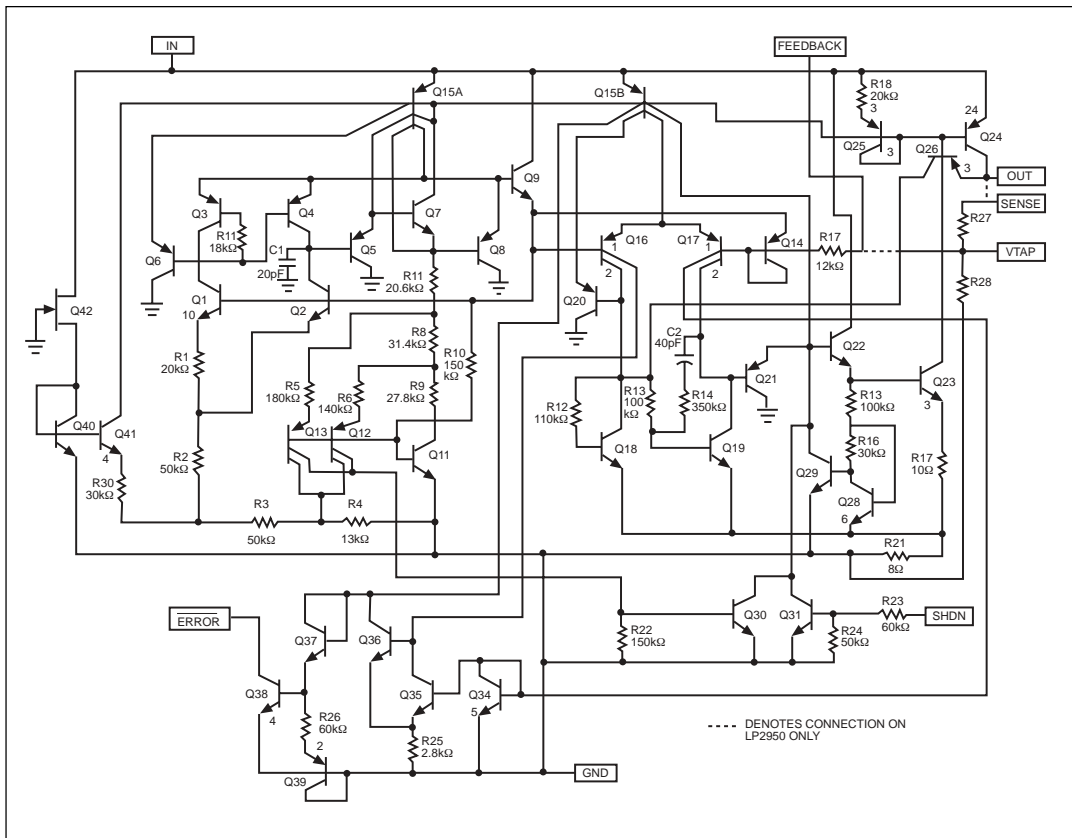
Figure 10. Schematic Diagram
