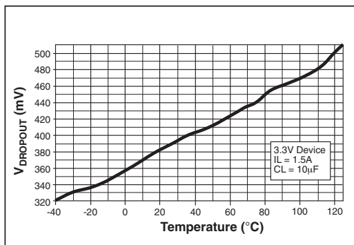
Figure 16. Dropout Voltage vs Temperature at I_{LOAD}=1.5\text{A}
