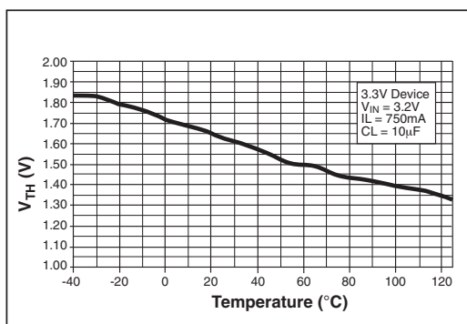
Figure 18. Enable Threshold vs Temperature for 3.3V Devices
