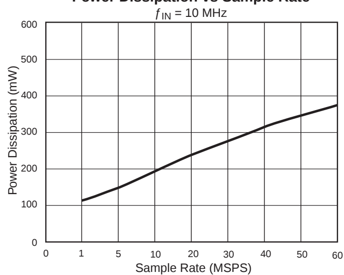
Power Dissipation vs Sample Rate
