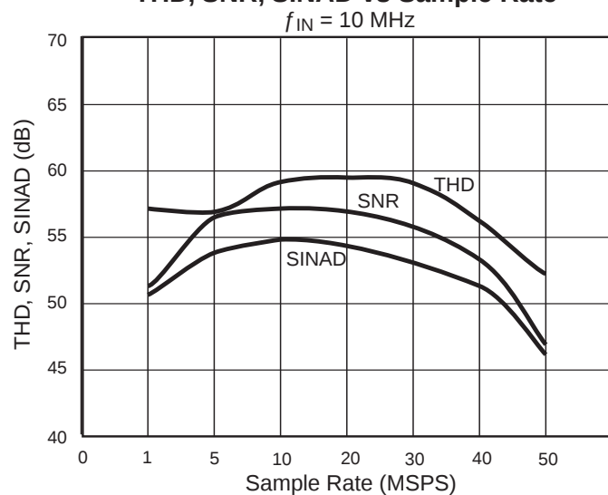
THD, SNR, SINAD vs Sample Rate
