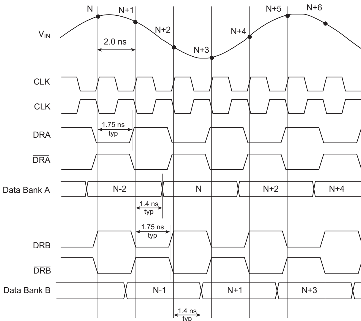
Figure 2 – Timing Diagram
