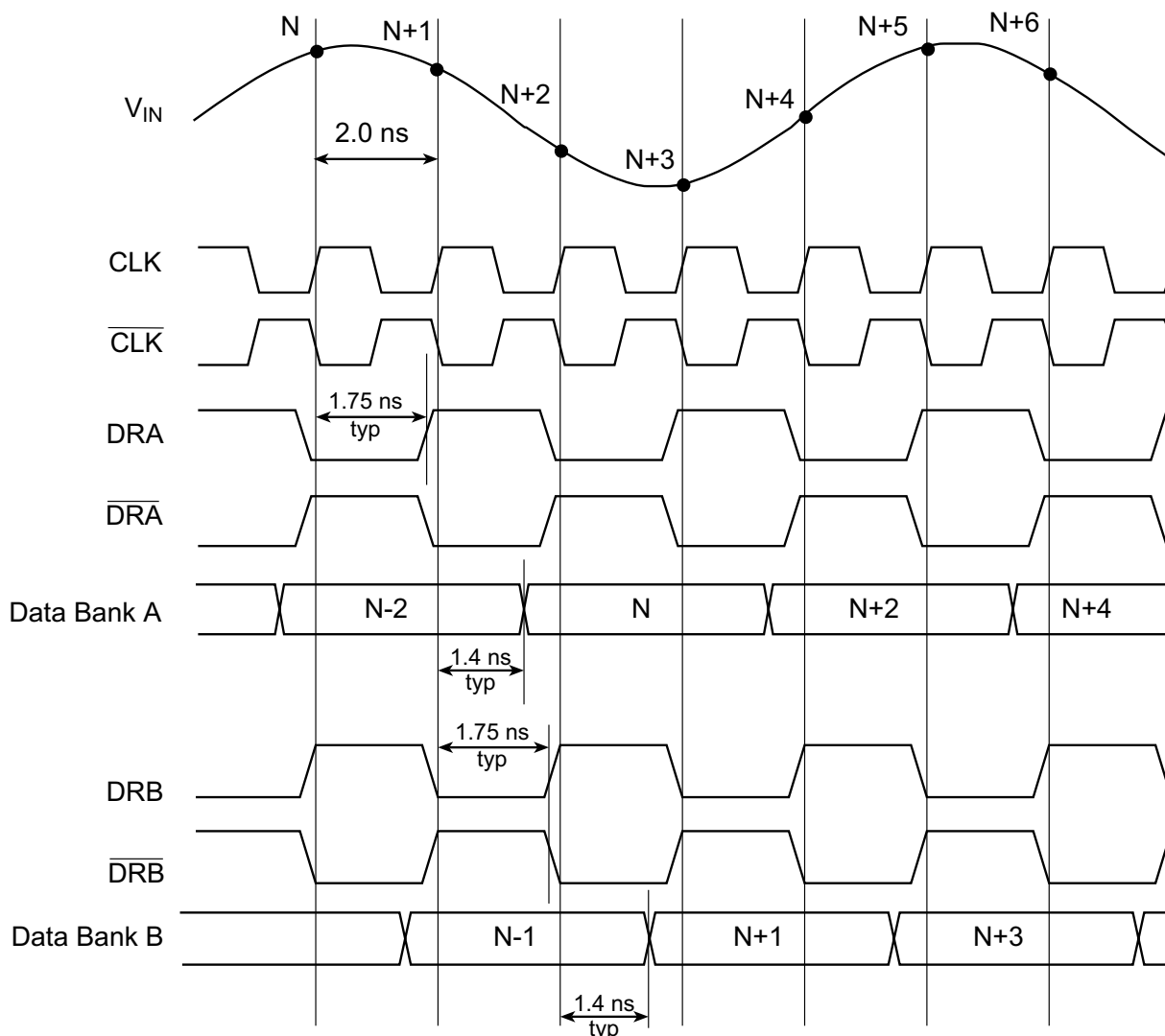
Figure 2 – Timing Diagram
