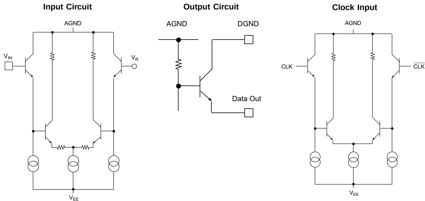
Figure 3 – Subcircuit Schematics
