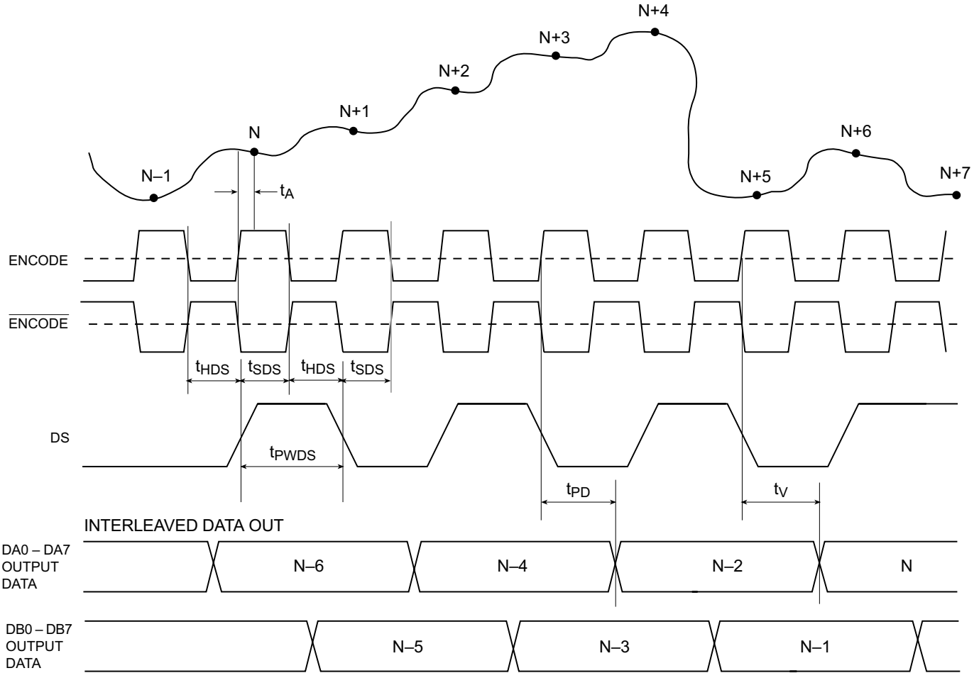
Figure 2 – Timing Diagram – Dual-Channel Mode
