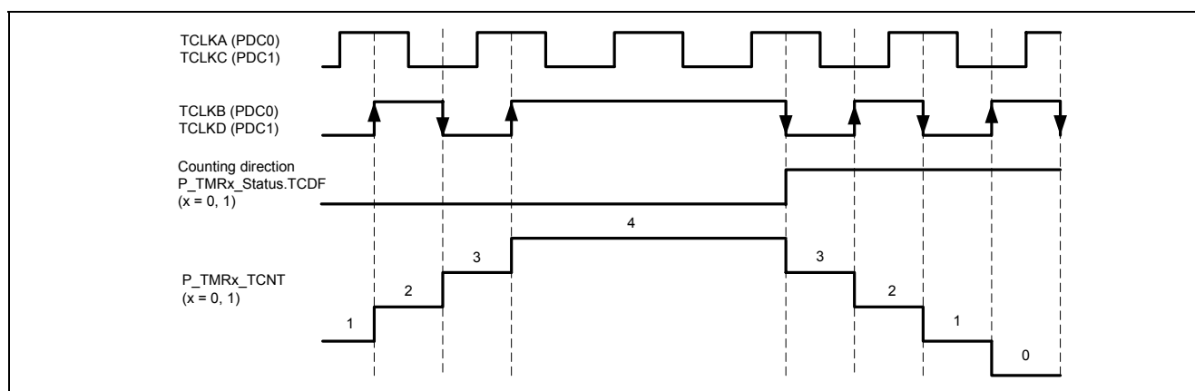
Figure 5-38 phase counting mode 4
