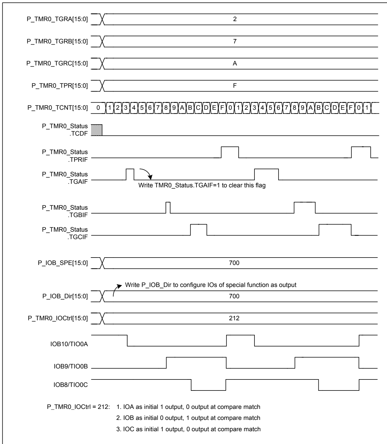
Figure 5-27 TMR0 edge aligned PWM
