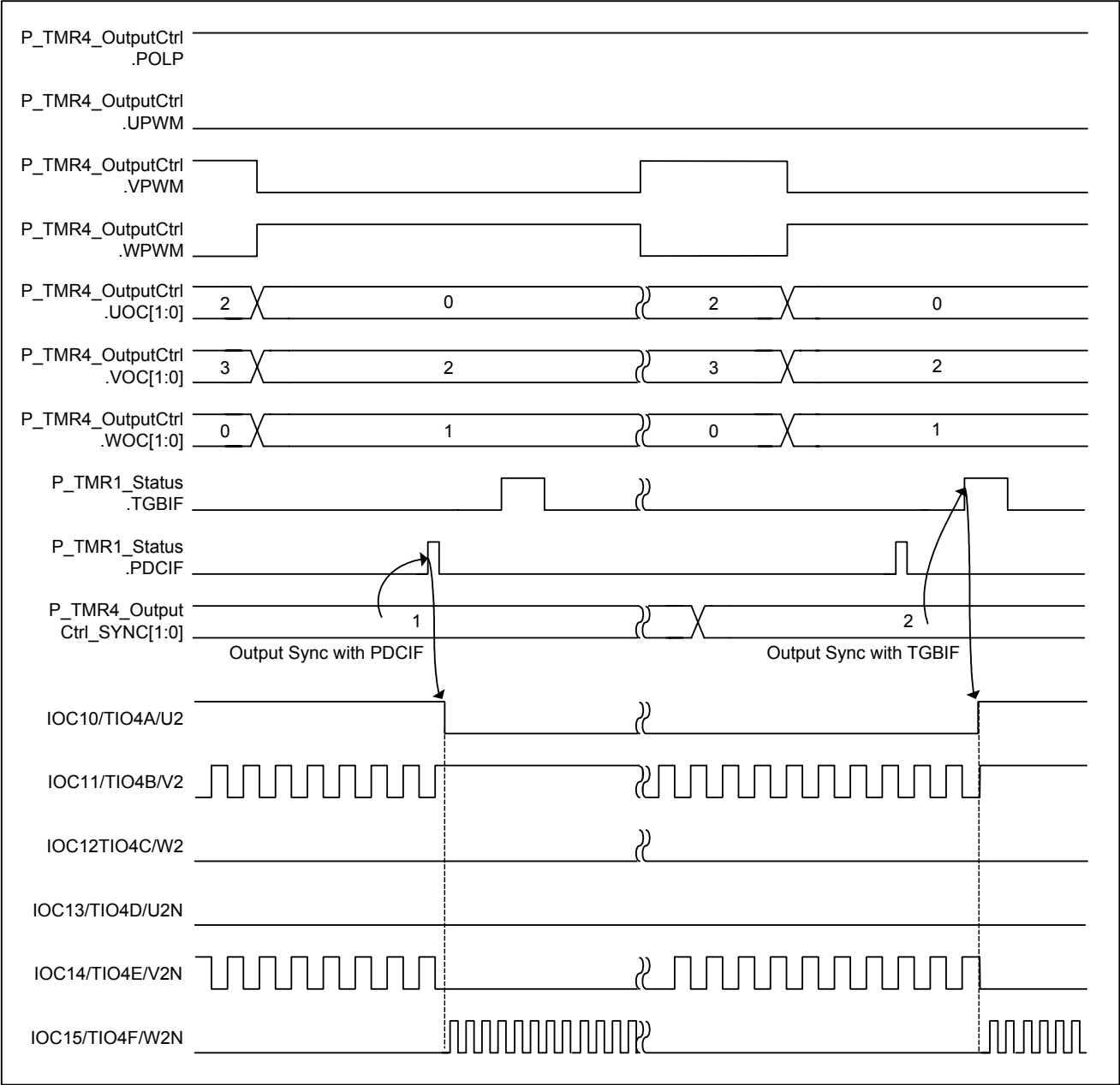
Figure 5-62 PWM Sync mode
