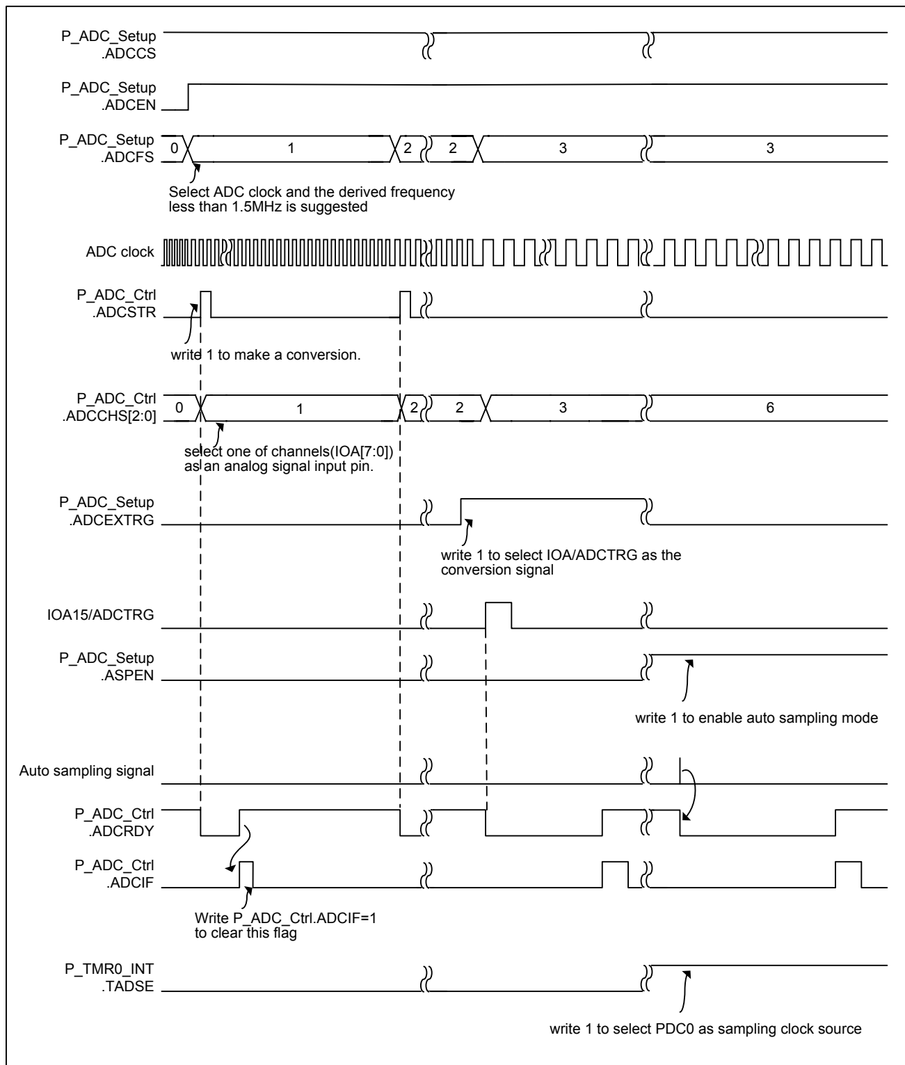
Figure 5-85 AD conversion timing
