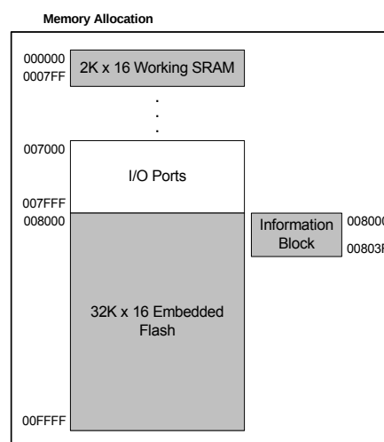
Figure 5-1 Memory allocation
