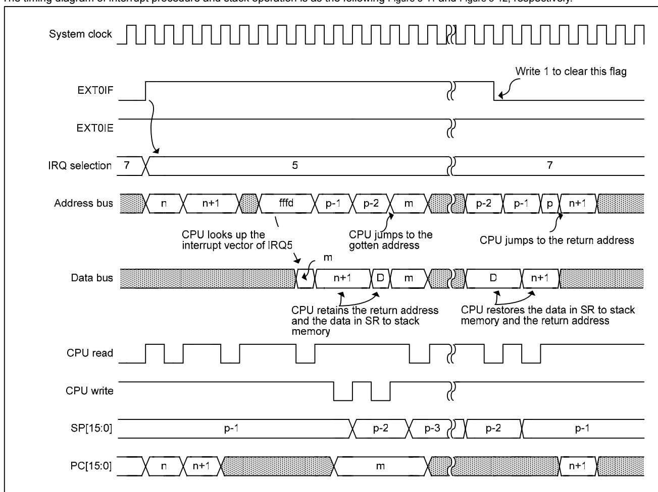
Figure 5-11 Interrupt procedure timing
