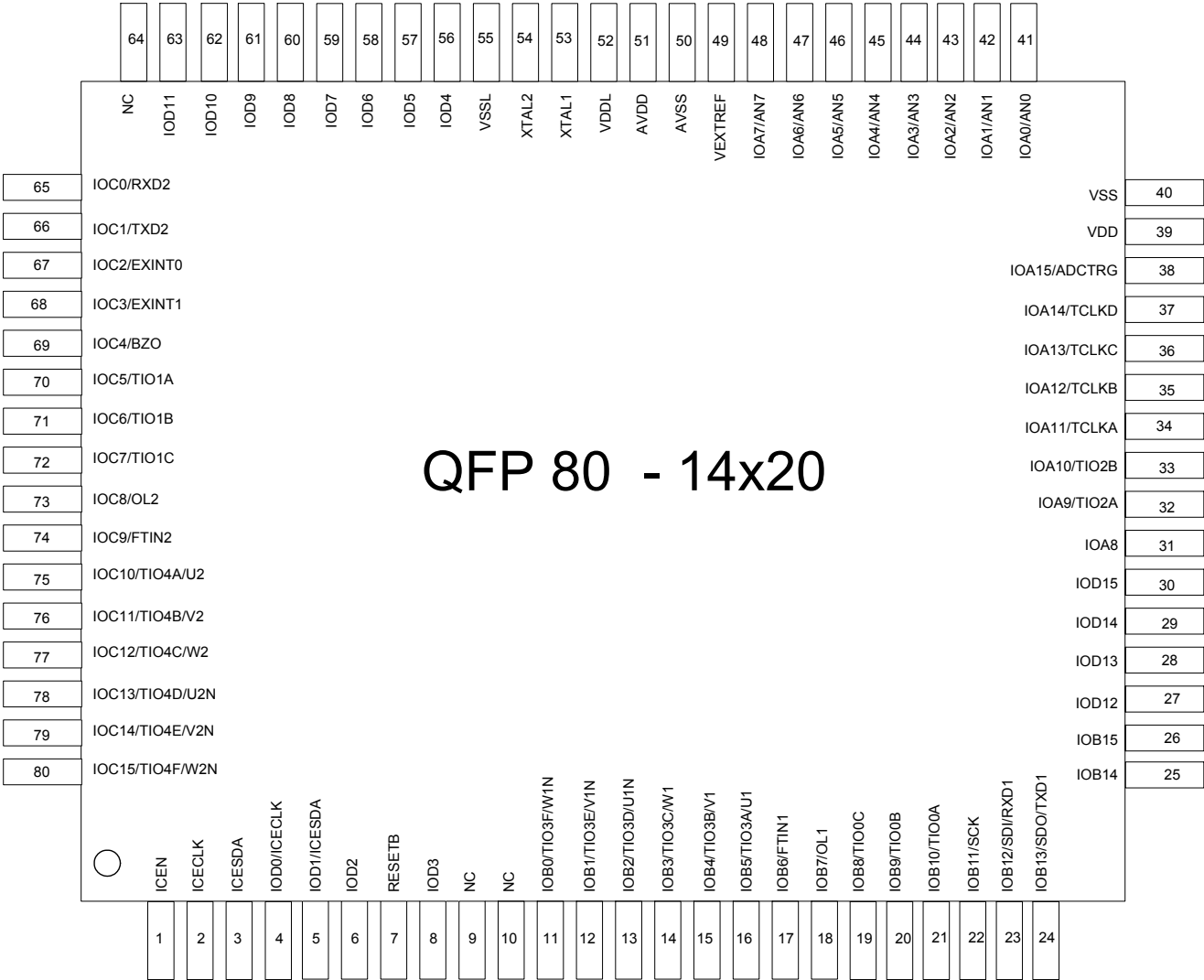
Figure 4-1 SPMC75F2413A QFP80 package
