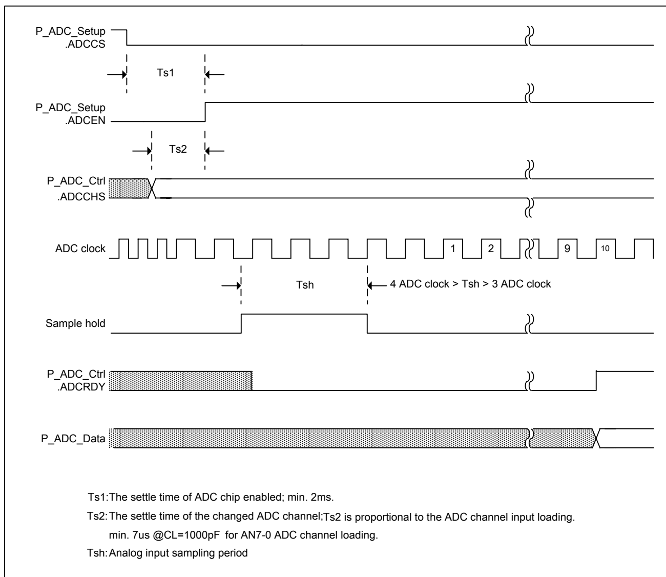
Figure 5-84 ADC timing diagram
