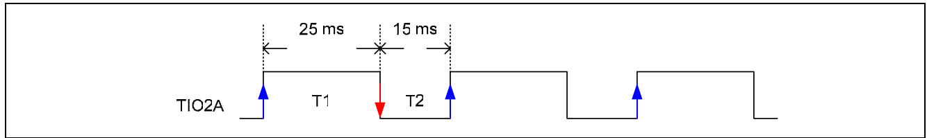
Figure 5-51 input capture signal connected to TIO2A
