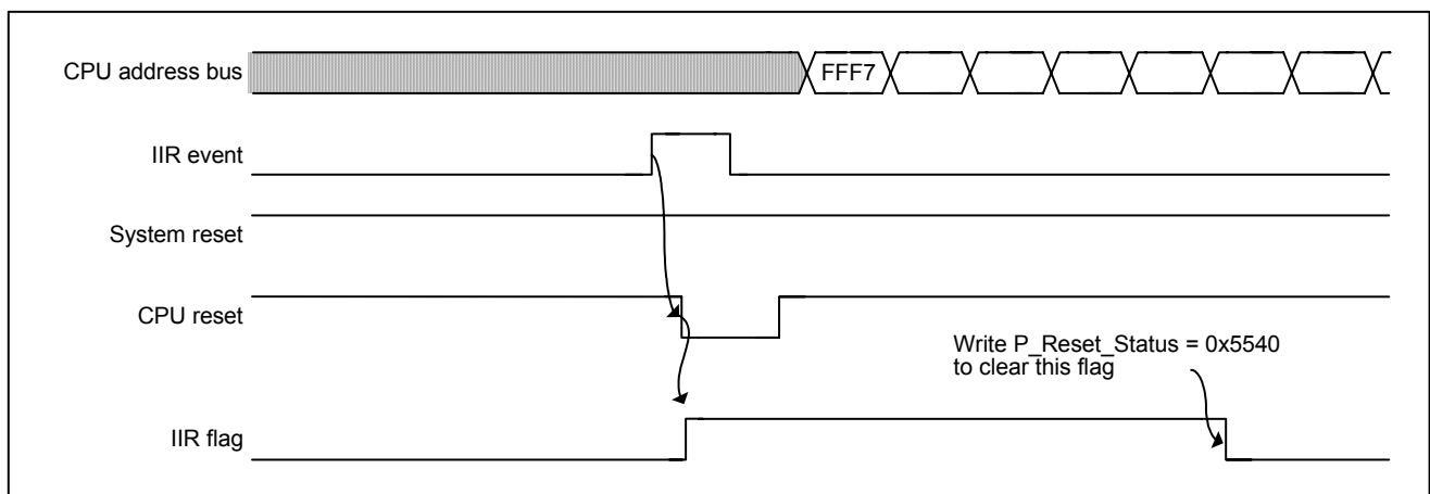
Figure 5-18 Illegal instruction reset timing
