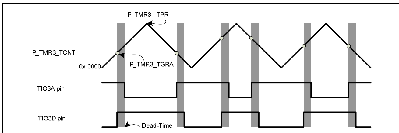
Figure 5-64 Active-low PWM mode of dead-time generation
