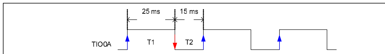
Figure 5-32 input capture signal connected to TIO0A
