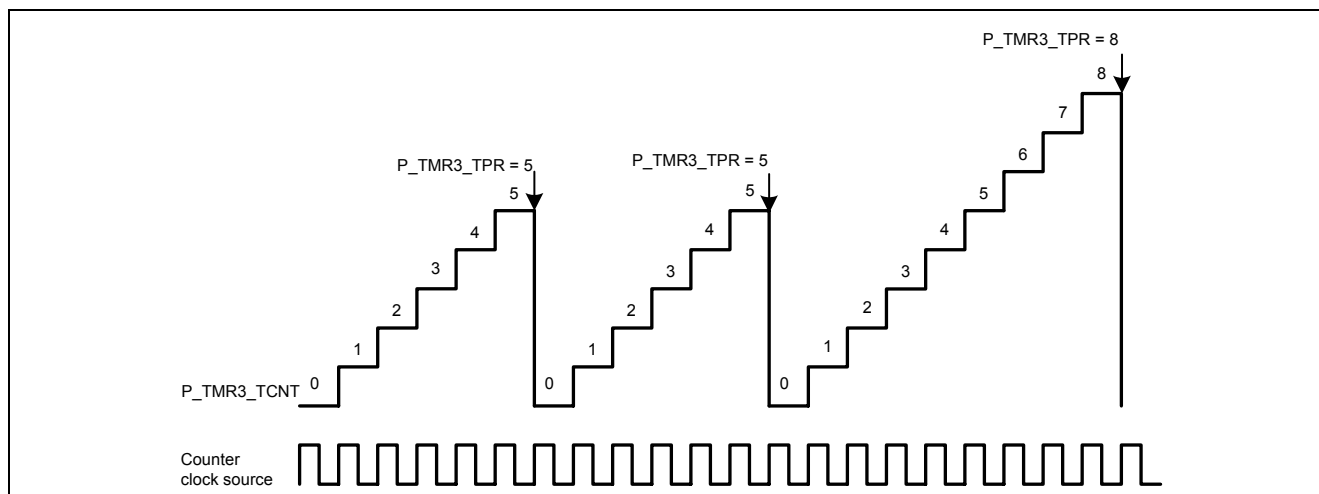
Figure 5-55 Continuous up counting example (CCLS = 111'b, CKEGS = 00'b, TMRPS = 000'b)
