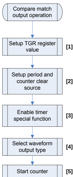
Figure 5-26 Example programming flowchart of PWM compare match output operation
