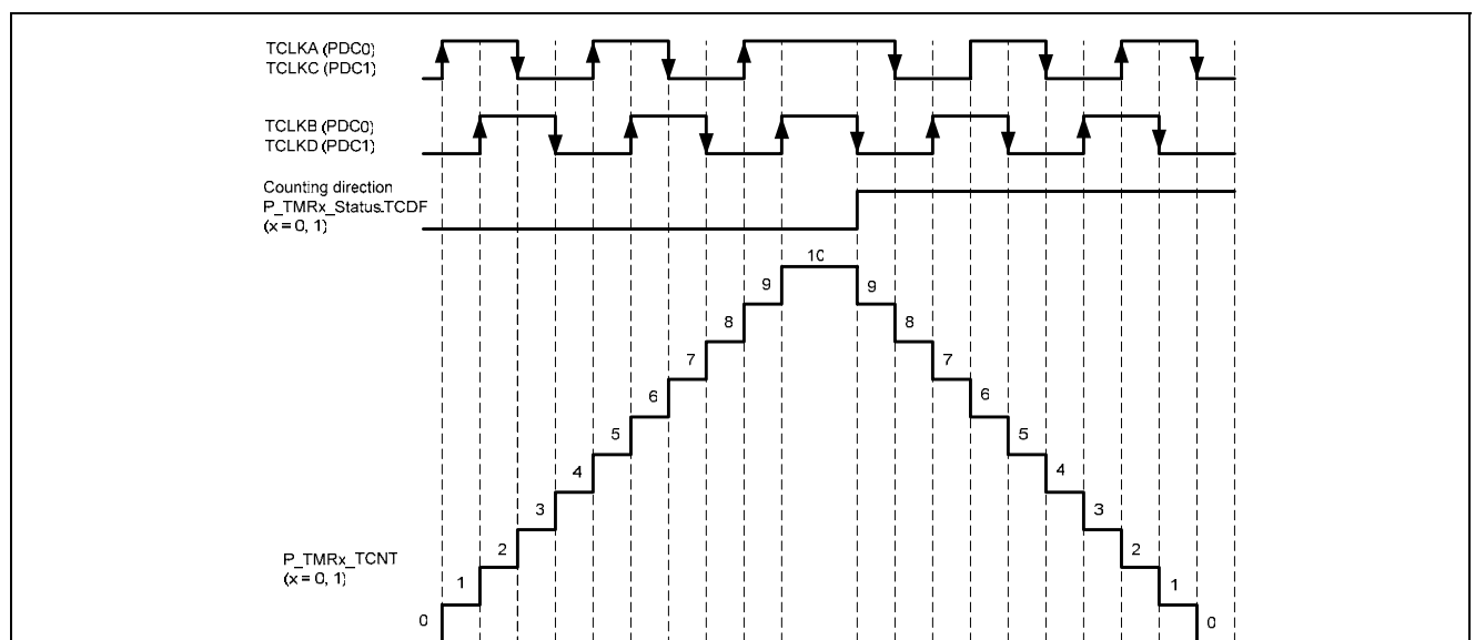
Figure 5-35 phase counting mode 1
