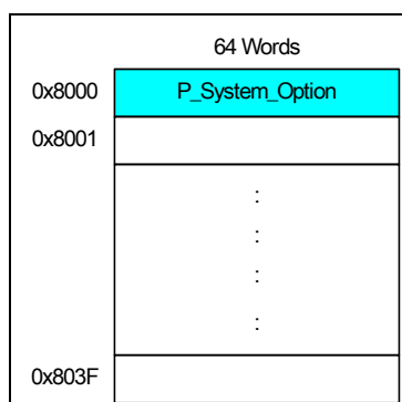
Figure 5-2 Structure of Information block
