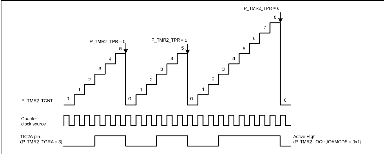
Figure 5-44 Edge-Aligned mode PWM
