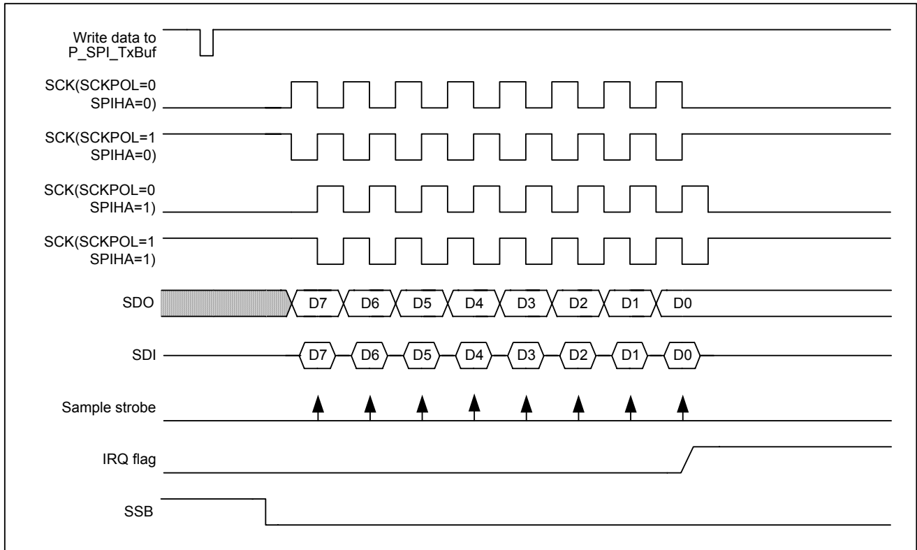
Figure 5-74 SPI mode timing, Slave Mode, SPIPHA = 0
