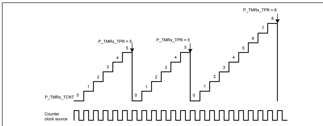
Figure 5-23 Continuous up counting example (CCLS = 111'b, CKEGS = 00'b, TMRPS = 000'b)
