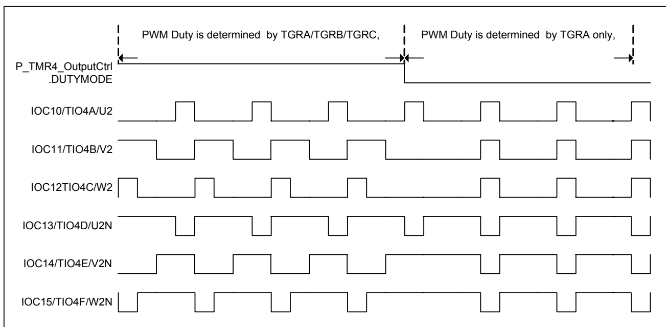
Figure 5-60 PWM output timing with different duty mode selection
