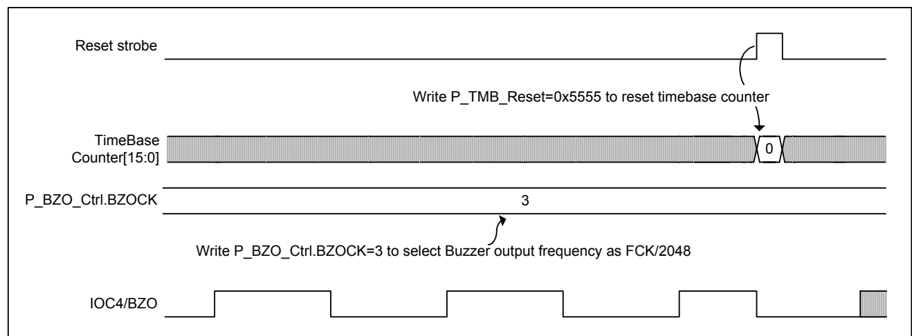
Figure 5-71 Timebase and buzzer output timing
