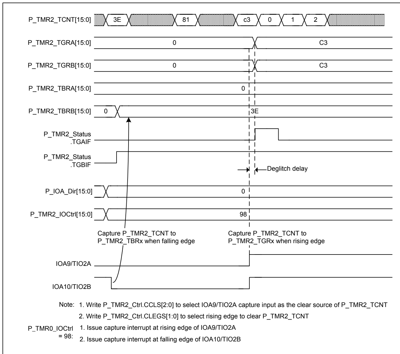
Figure 5-53 Capture input signal width and cycle
