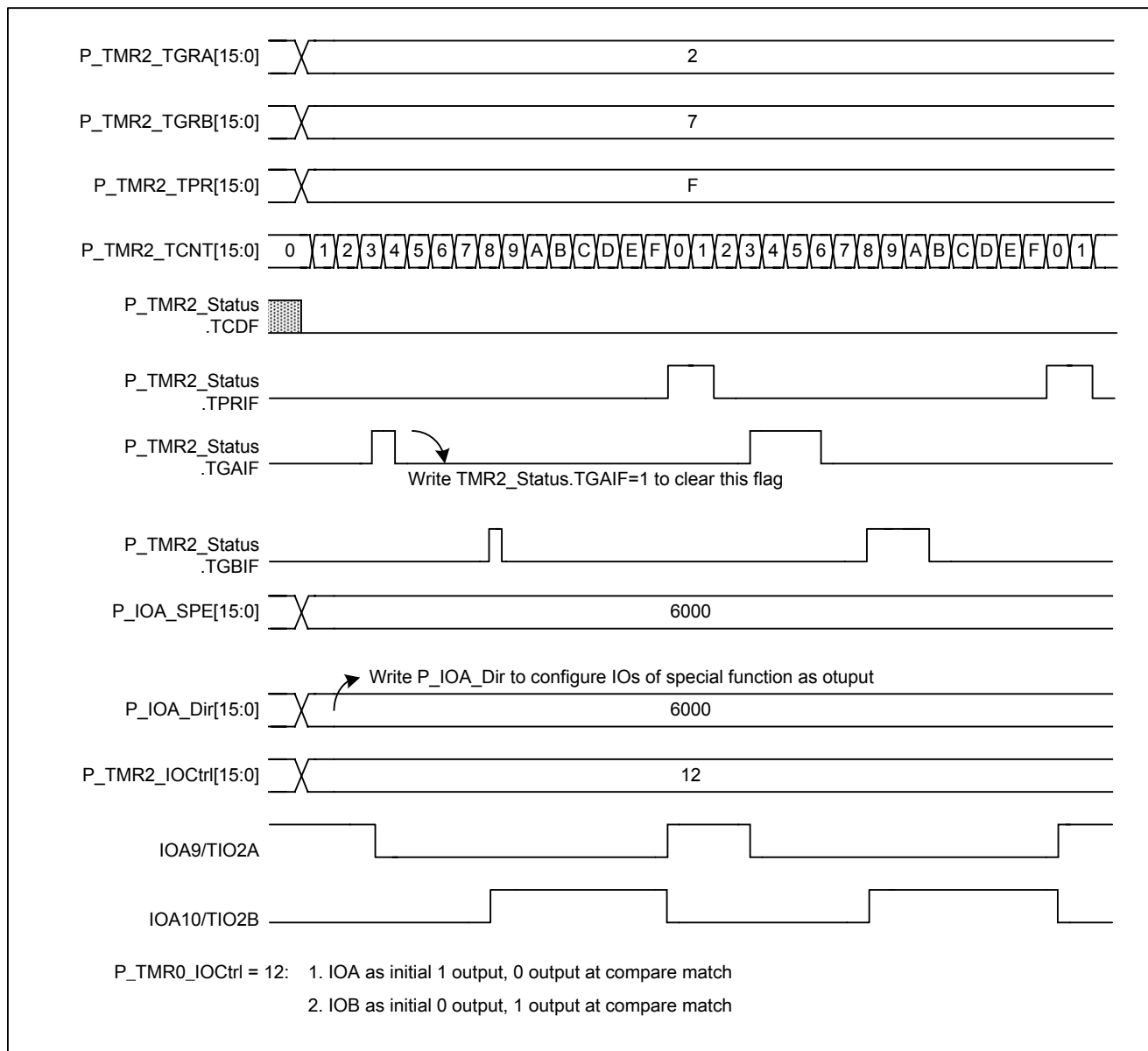
Figure 5-46 TMR2 edge aligned PWM
