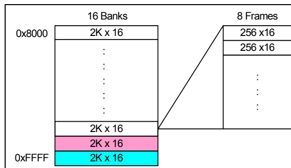
Figure 5-3 Page0 and frame of flash
