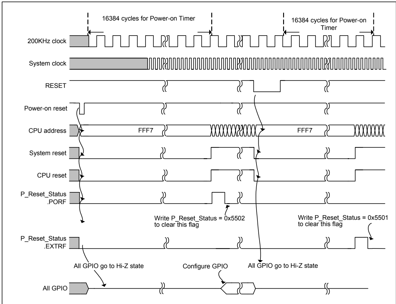
Figure 5-14 Power-on reset, external reset and power-up timer timing
