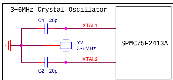
Figure 5-5 The crystal circuit connection
