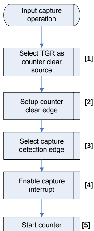
Figure 5-33 Example programming flowchart of input capture operation
