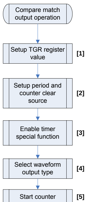
Figure 5-45 Example programming flowchart of PWM compare match output operation
