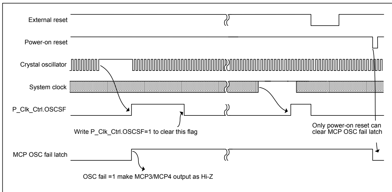
Figure 5-8 Clock Fail timing
