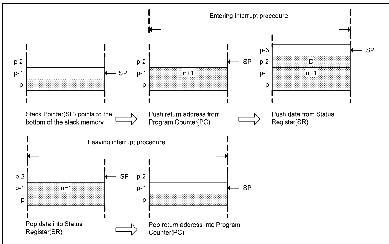
Figure 5-12 Stack memory operation with interrupt procedure
