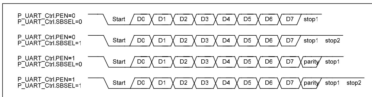
Figure 5-76 UART Data Format
