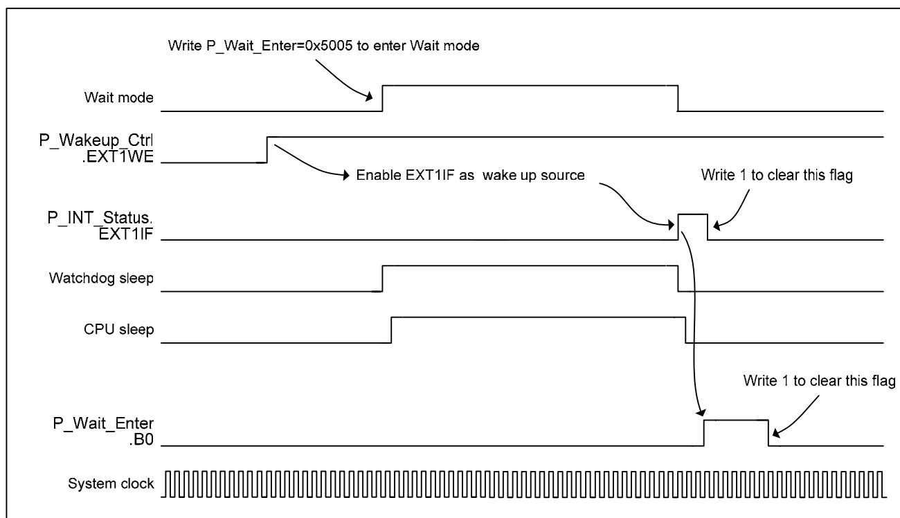
Figure 5-9 Wait mode timing
