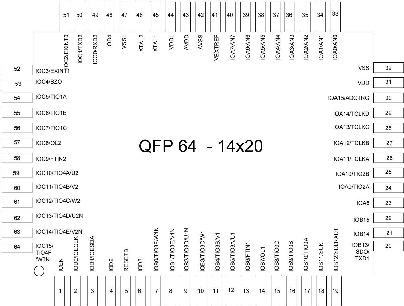
Figure 4-2 SPMC75F2413A QFP64 package
