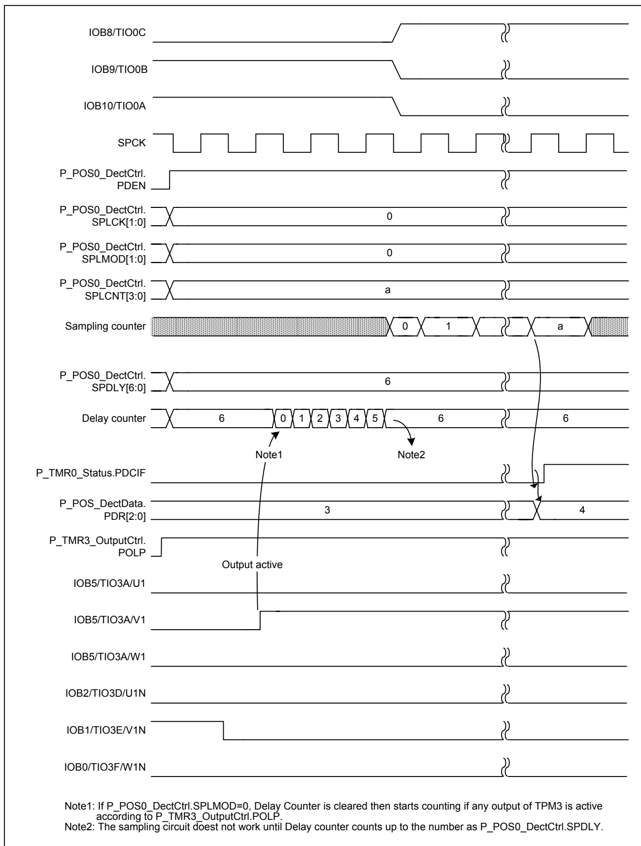
Figure 5-41 Position detection with noise filter
