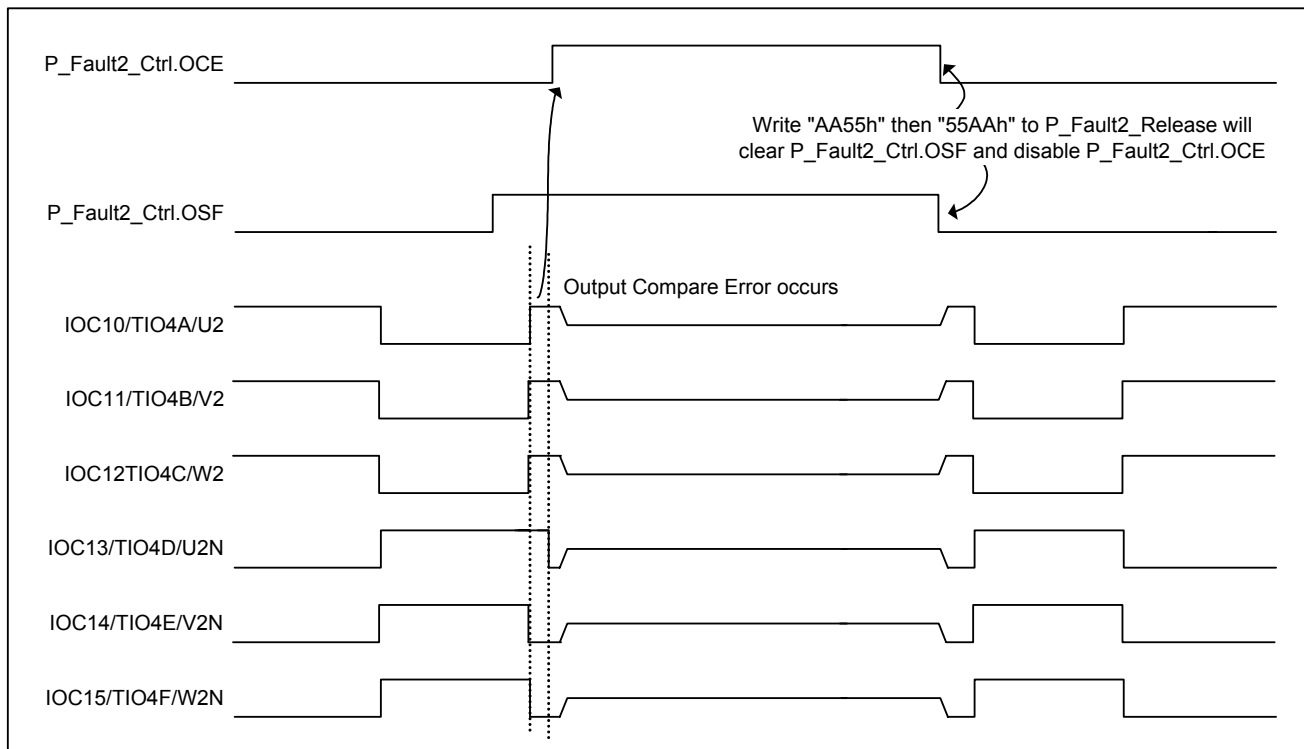
Figure 5-66 Output compare error
