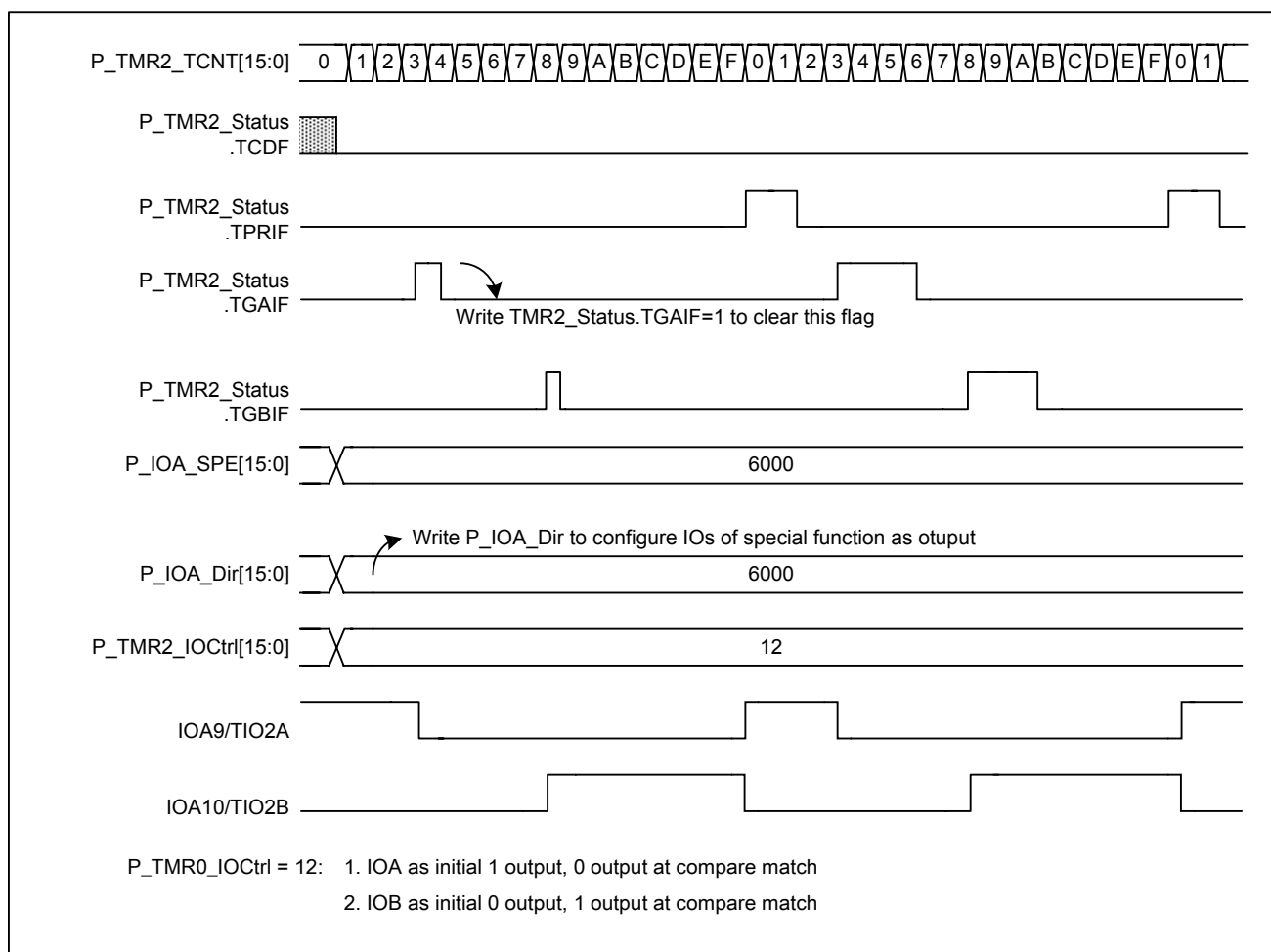
Figure 5-47 Timer mode output timing
