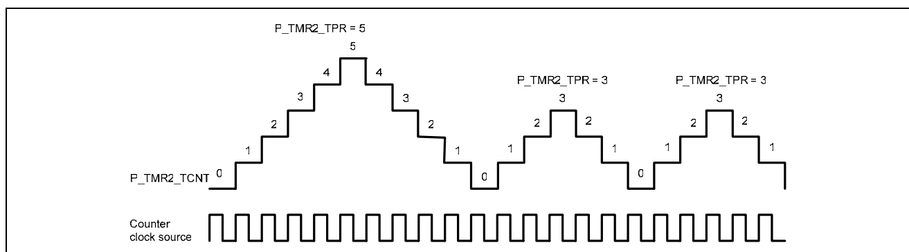
Figure 5-49 Center-Aligned mode PWM
