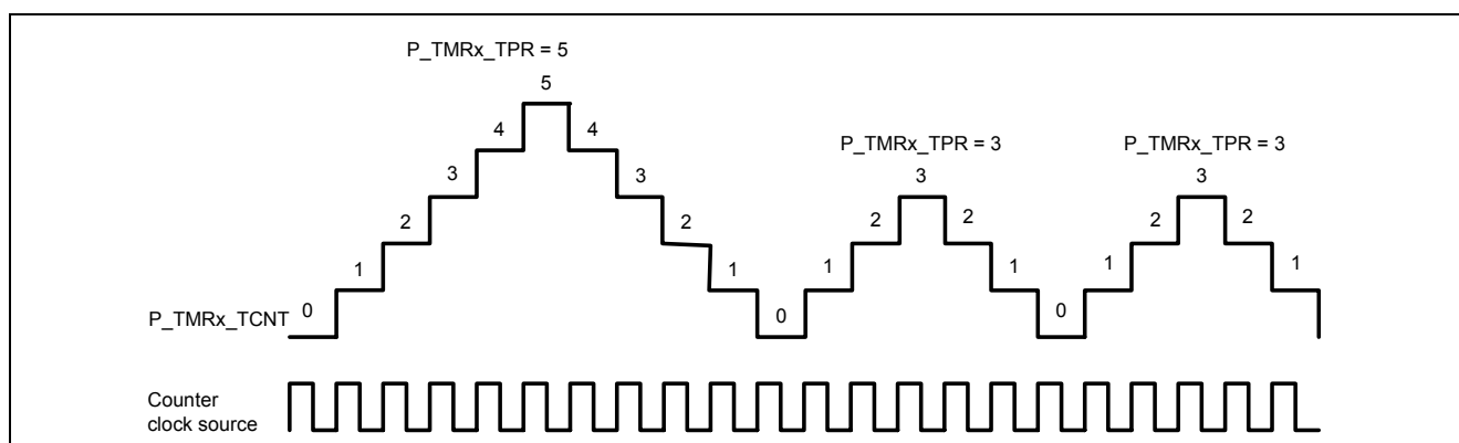
Figure 5-57 Continuous up/down counting example (CCLS = 111'b, CKEGS = 00'b, TMRPS = 000'b)
