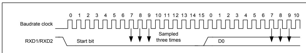
Figure 5-78 Data sampling scheme
