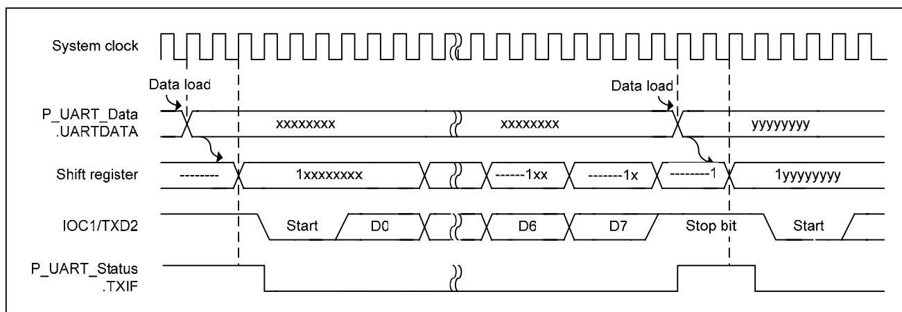
Figure 5-77 Data Transmission Timing
