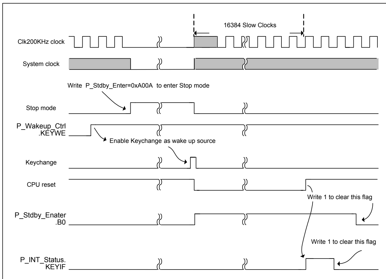
Figure 5-10 Standby mode timing
