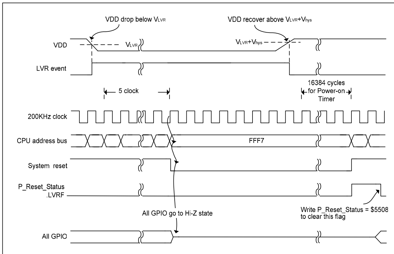
Figure 5-15 Low voltage reset timing
