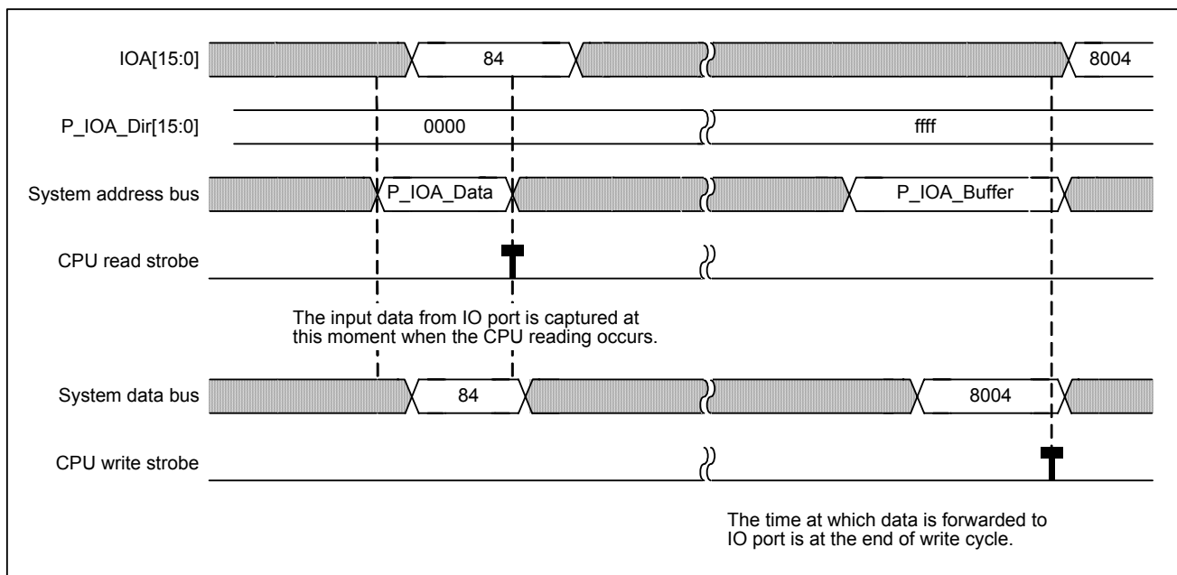
Figure 5-20 GPIO input/output timing
