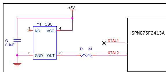
Figure 5-7 The external clock from oscillator connection
