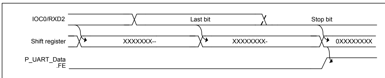
Figure 5-82 Frame Error timing
