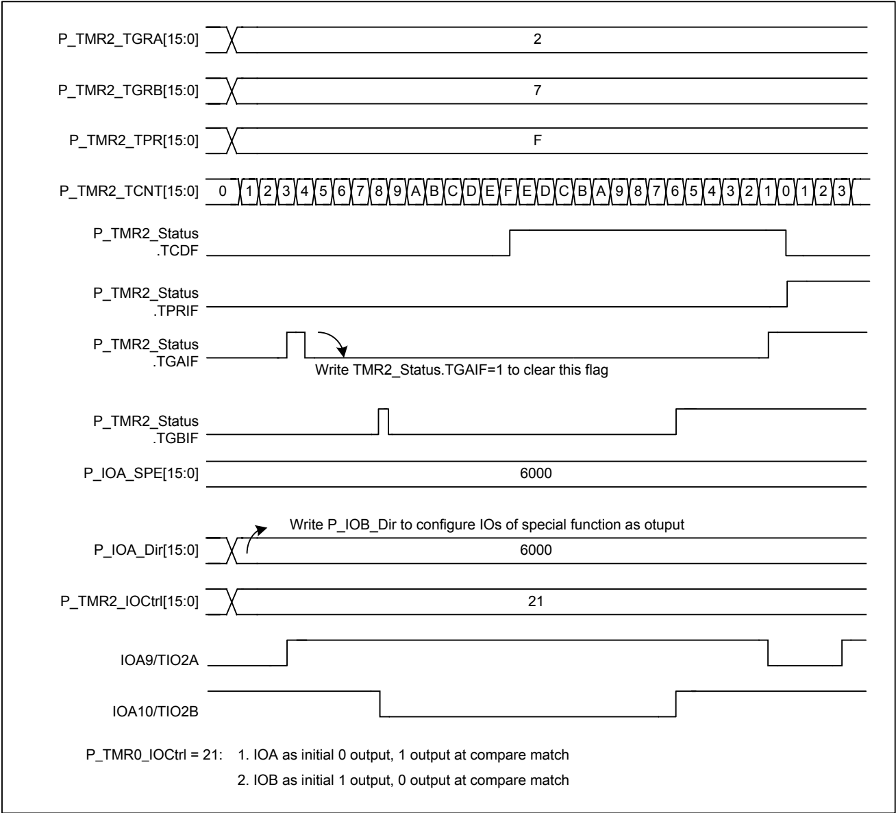
Figure 5-50 TMR2 center aligned PWM
