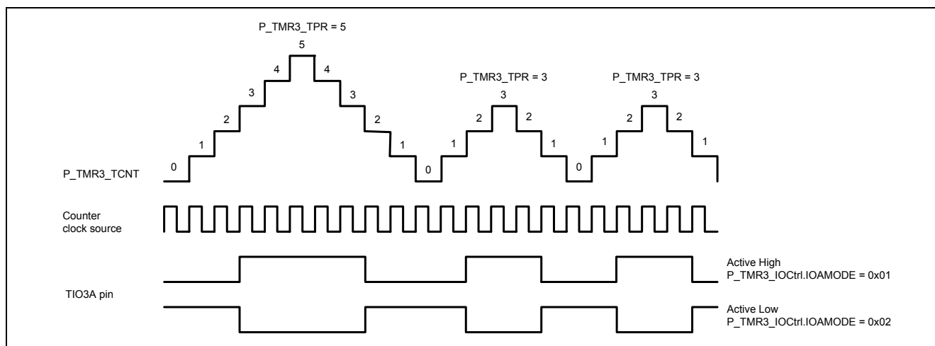
Figure 5-58 Center-Aligned mode PWM
