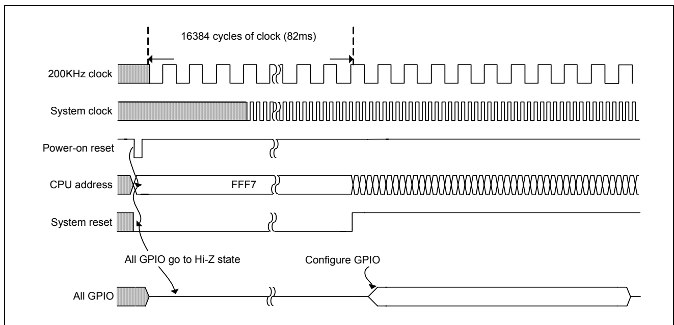
Figure 5-4 Power-up procedure
