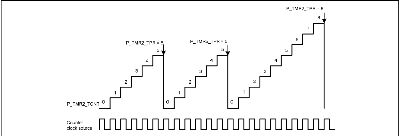
Figure 5-43 Continuous up counting example (CCLS = 111'b, CKEGS = 00'b, TMRPS = 000'b)
