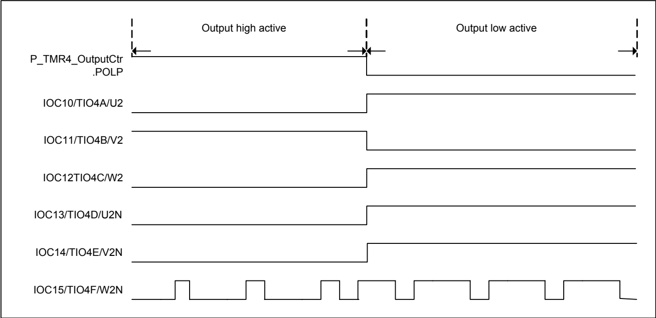
Figure 5-61 Output polarity timing
