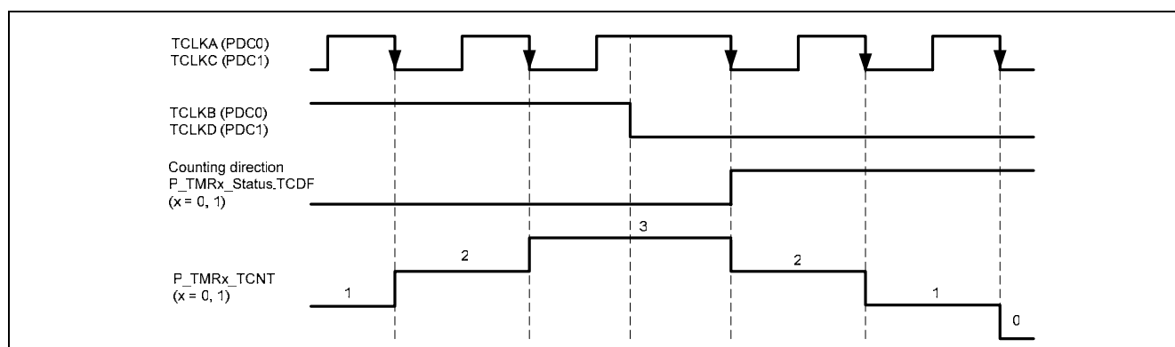
Figure 5-36 phase counting mode 2
