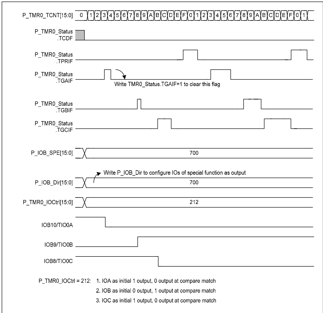
Figure 5-28 Timer mode output timing
