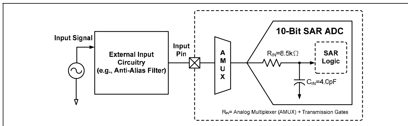
Figure 5-83 ADC equivalent circuit for SPMC75F2413A
