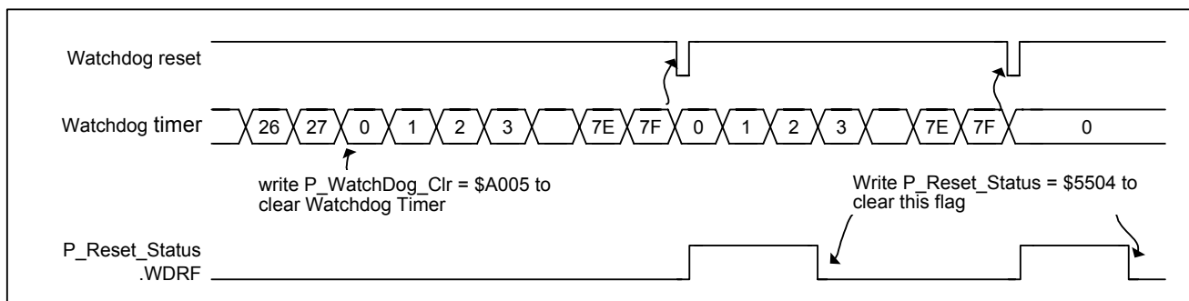
Figure 5-16 Watchdog timer reset timing
