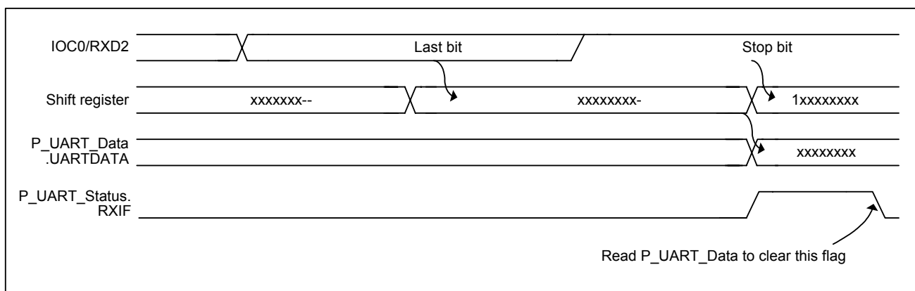
Figure 5-79 RX buffer full
