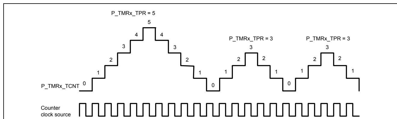
Figure 5-29 Continuous up/down counting example (CCLS = 111'b, CKEGS = 00'b, TMRPS = 000'b)
