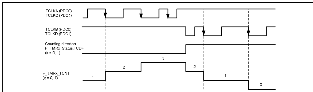
Figure 5-37 phase counting mode 3
