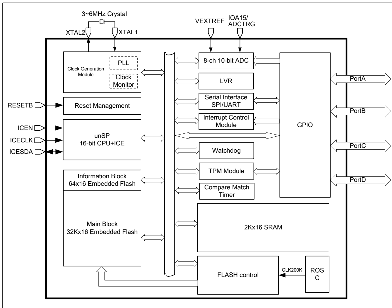
Figure 3-1 SPMC75F2413A function block diagram
