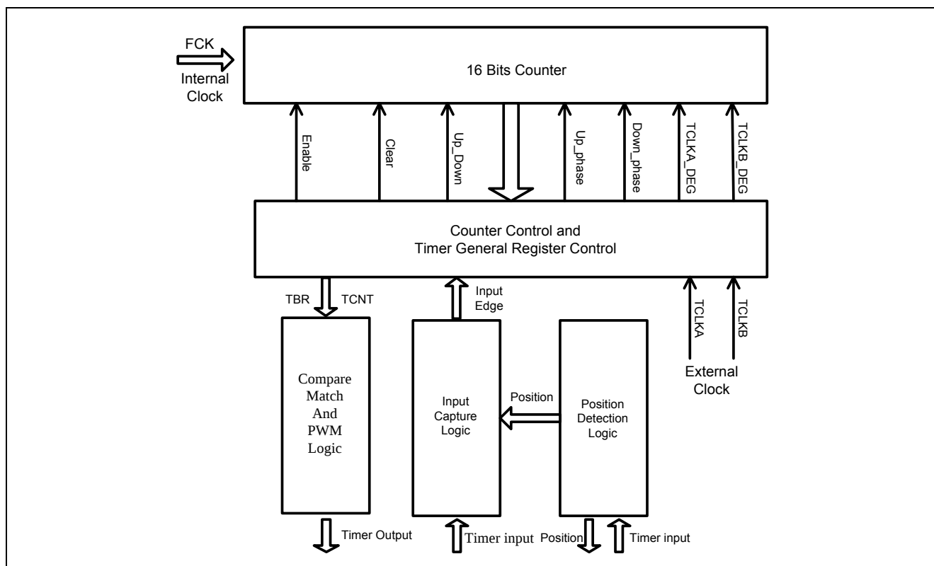
Figure 5-22 PDC timers block diagram
