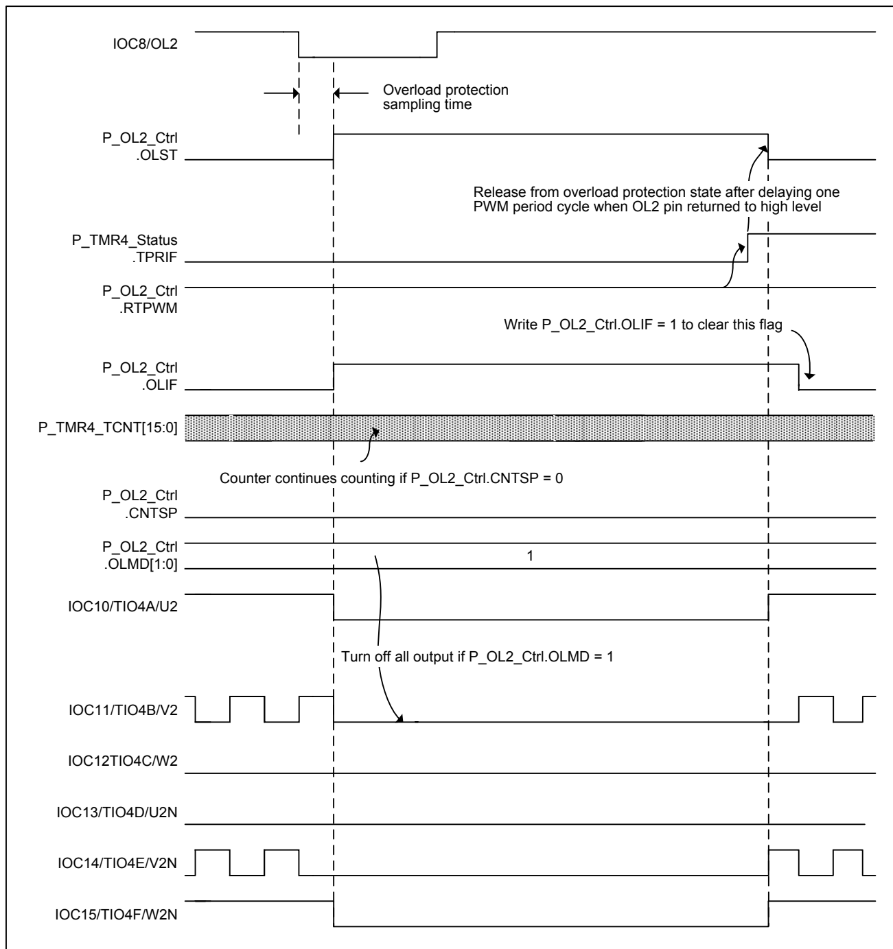
Figure 5-69 Stop all output when overload occurs
