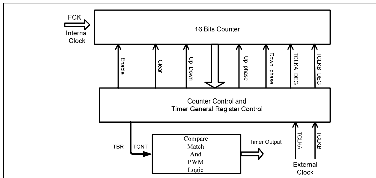
Figure 5-42 TPM timer 2 block diagram
