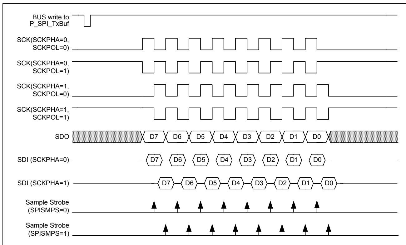
Figure 5-73 SPI mode timing, Master Mode
