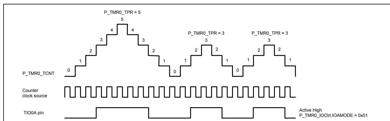
Figure 5-30 Center-aligned mode PWM
