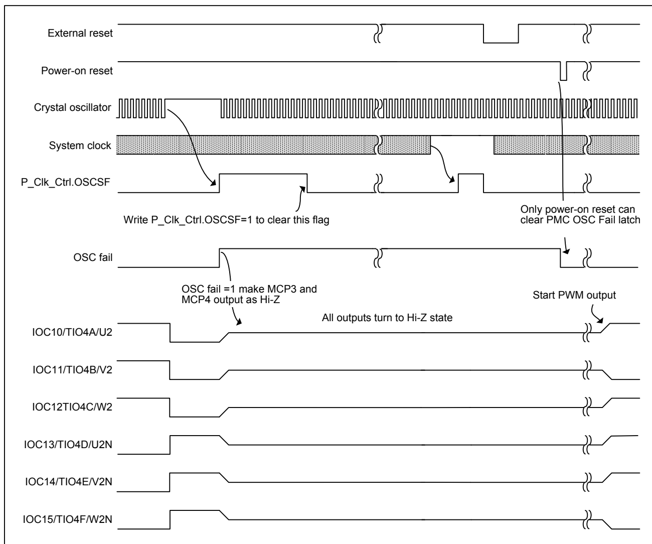
Figure 5-67 Oscillator stopped timing
