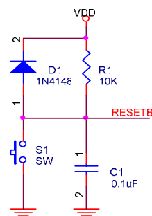
Figure 5-13 External reset circuit
