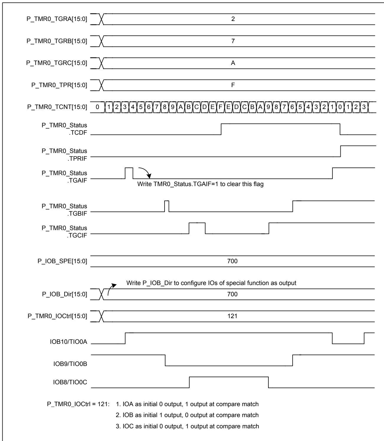
Figure 5-31 TMR0 center aligned PWM
