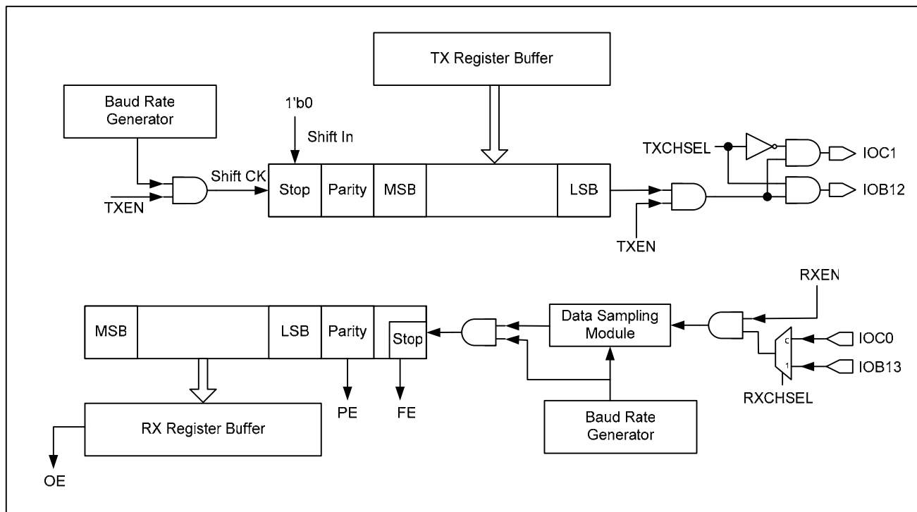
Figure 5-75 UART block diagram
