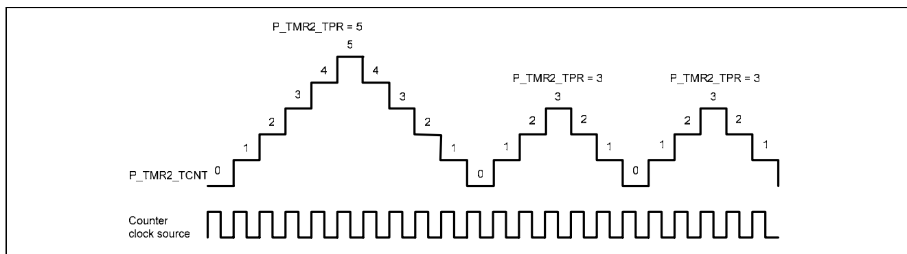
Figure 5-48 Continuous up/down counting example (CCLS = 111'b, CKEGS = 00'b, TMRPS = 000'b)
