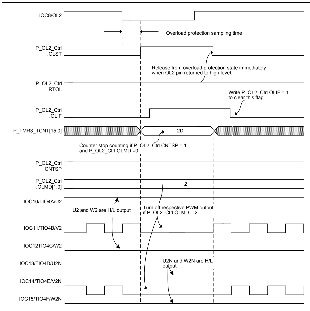
Figure 5-68 Stop PWM output only when overload occurs
