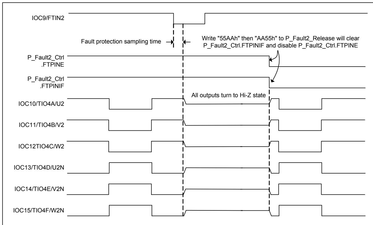
Figure 5-65 Fault error timing
