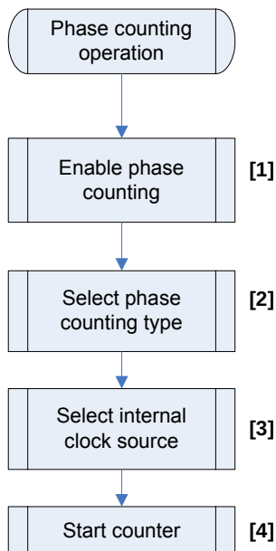
Figure 5-39 Example programming flowchart of phase counting operation
