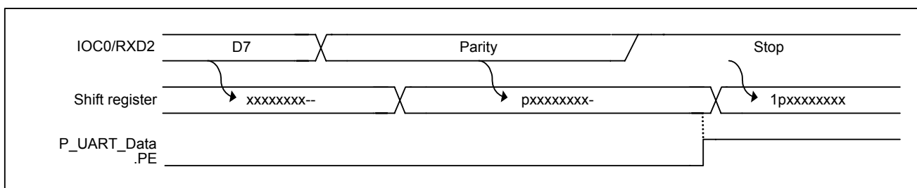
Figure 5-81 Parity Error timing
