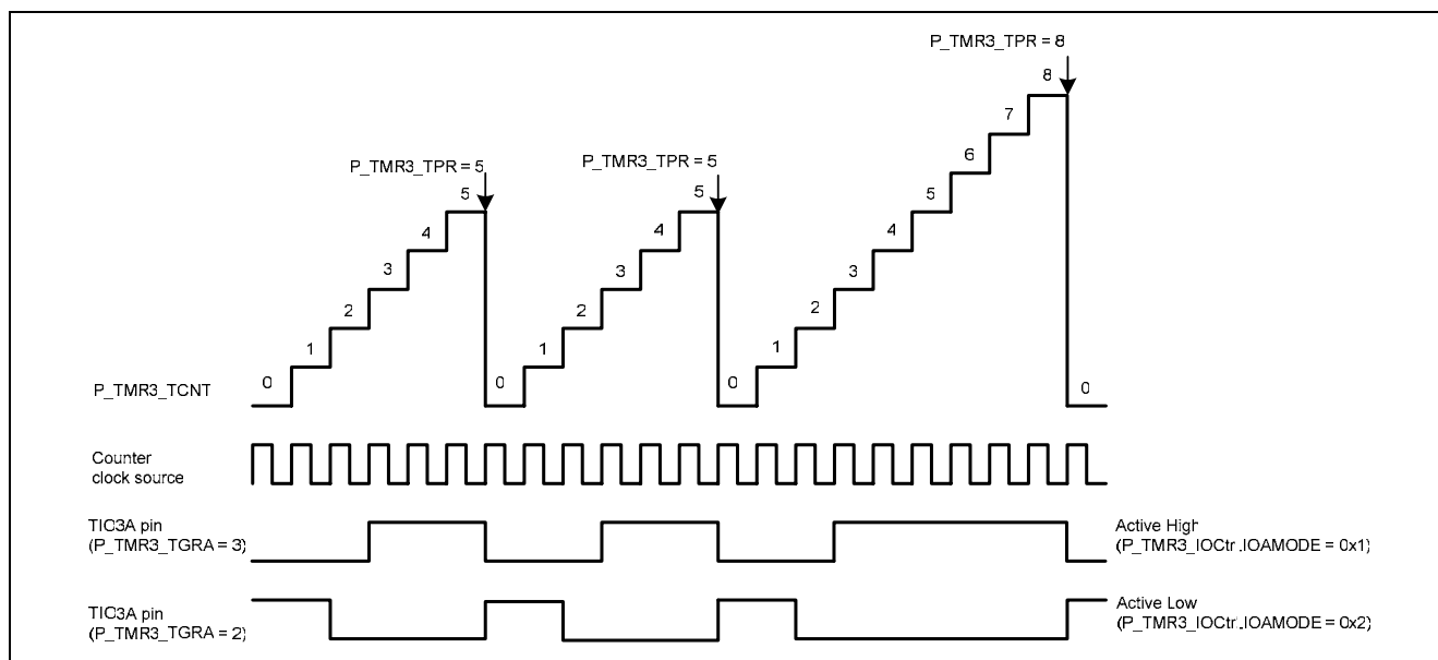
Figure 5-56 Edge-Aligned mode PWM
