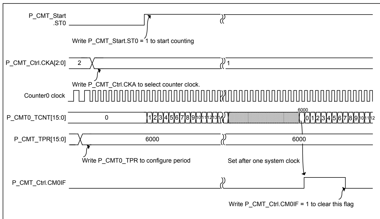
Figure 5-70 CMT timing
