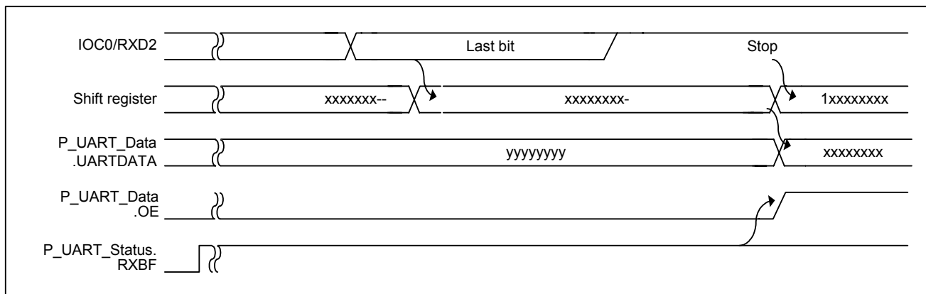
Figure 5-80 Overrun error timing
