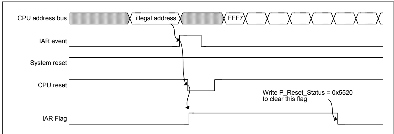
Figure 5-17 Illegal address reset timing
