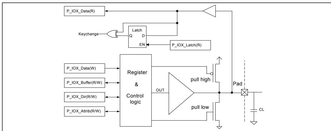
Figure 5-19 IO structure diagram
