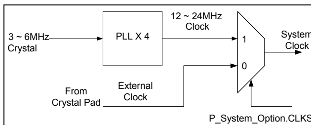
Figure 5-6 PLL and external clock block diagram
