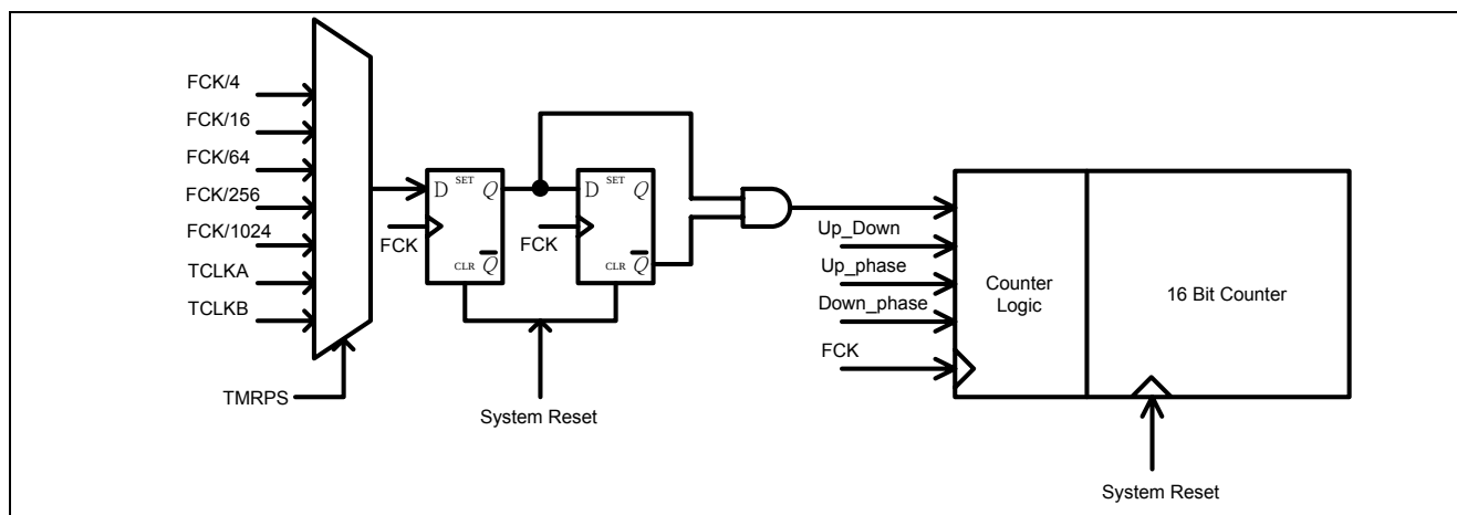
Figure 5-54 MCP timer 3 and 4 block diagram
