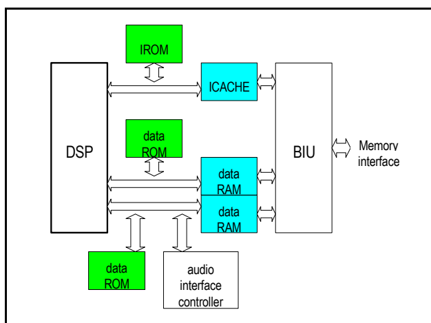
Figure 5-10: Audio DSP architecture
