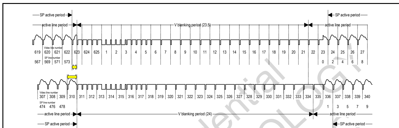
Figure 6-9: PAL (576i) timing diagram
