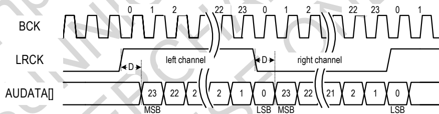
Figure 6-7: I²S mode / 24bit data / 24bit frame
