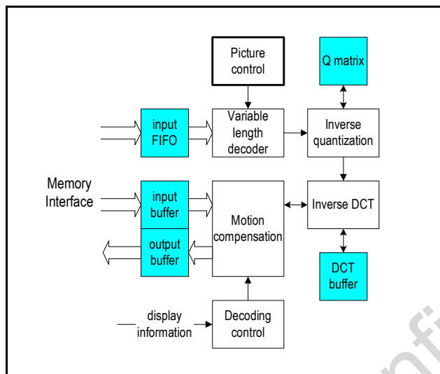
Figure 5-8: architecture of video decoding pipeline
