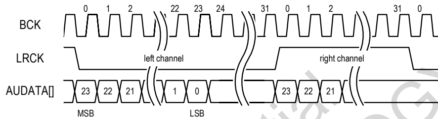
Figure 6-5: Left justified mode / 24bit data / 32bit frame / MSB first
