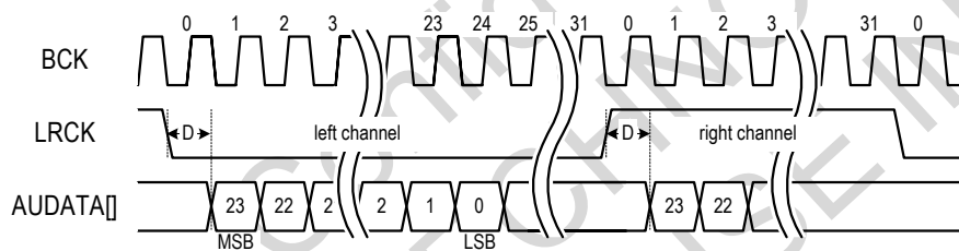
Figure 6-6: I²S mode / 24bit data / 32bit frame
