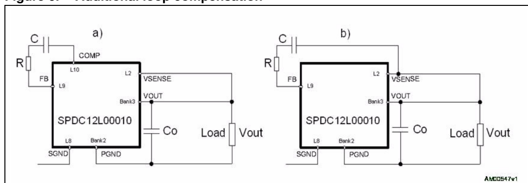
Figure 6. Additional loop compensation
