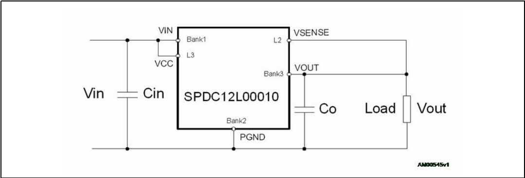
Figure 4. Voltage sensing
