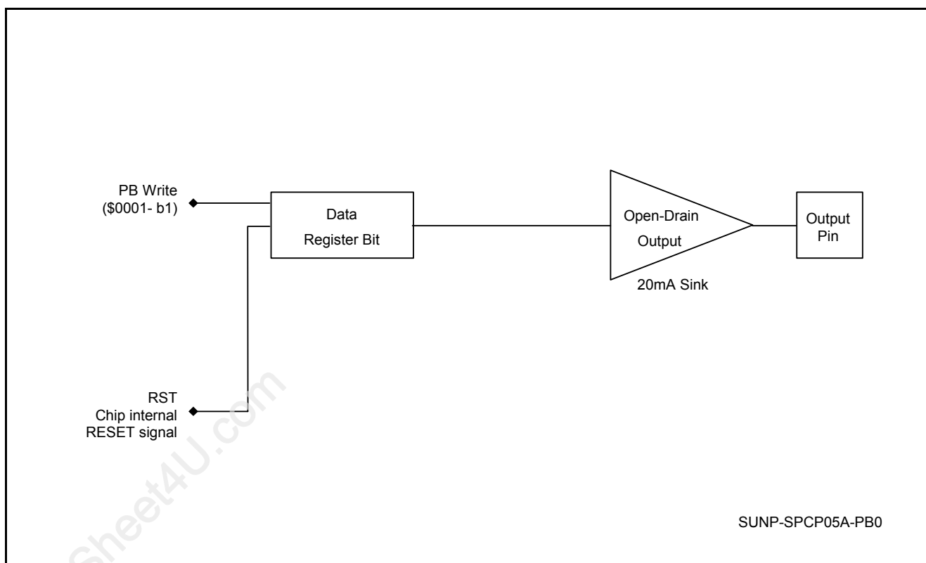
Figure 6. PB1 I/O Diagram
