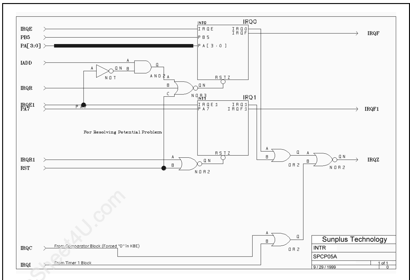
Figure 7. Interrupt Source Diagram
