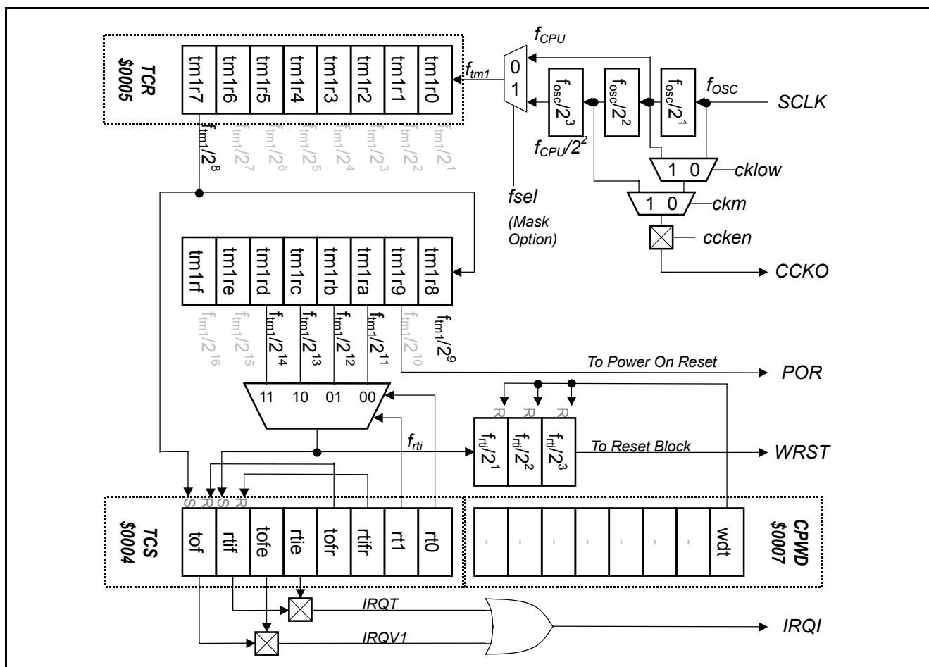
Figure 10. Block Diagram of WDT and Timer 1
