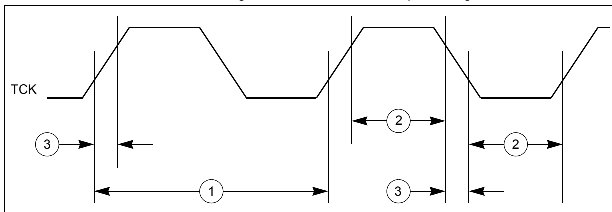
Figure 16. JTAG test clock input timing
