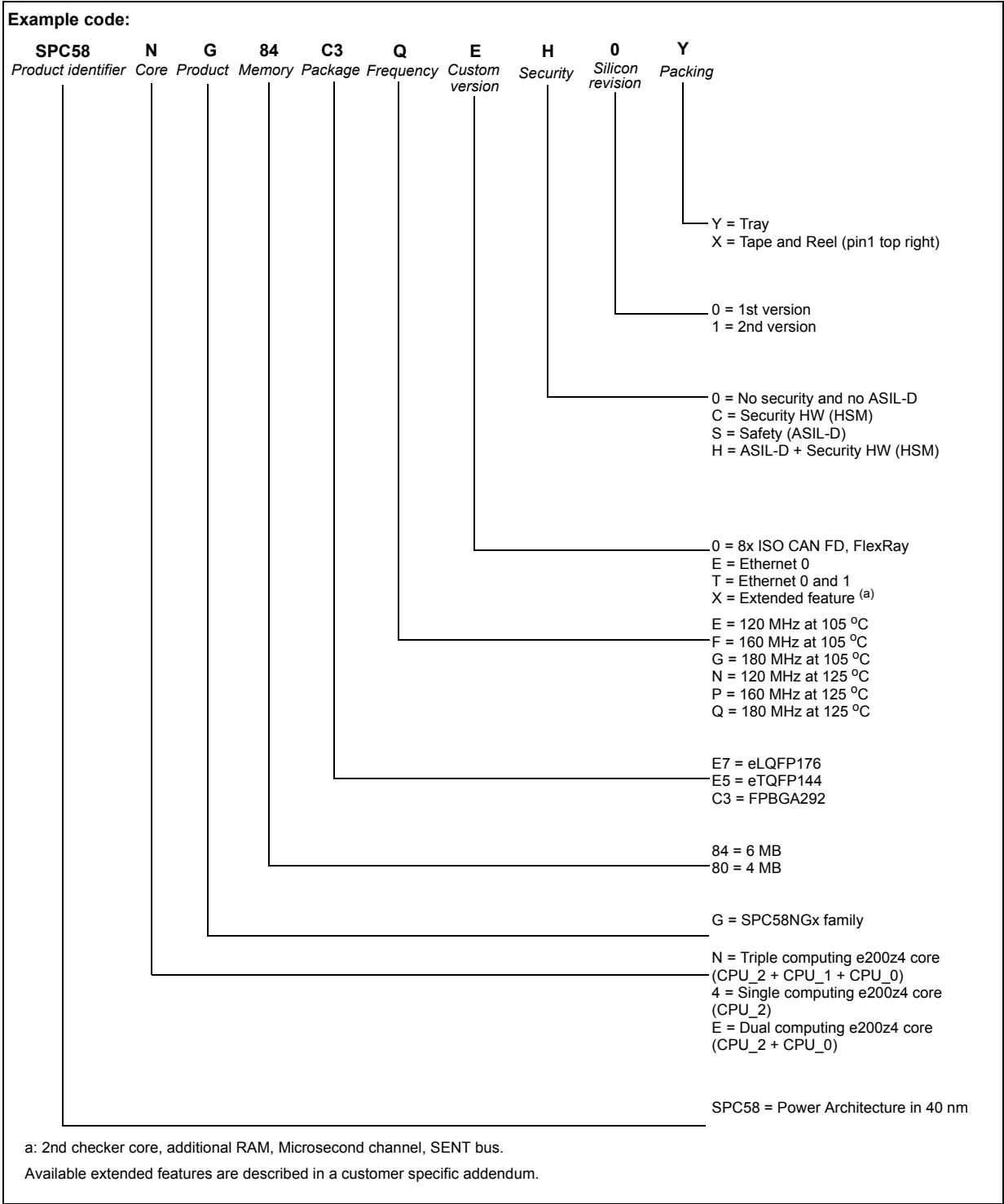
Figure 50. Ordering information scheme
