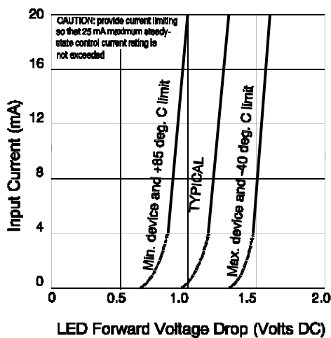
Figure 3. Input Characteristics (Current Controlled)
