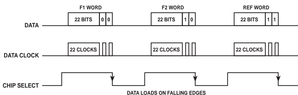
Fig. 7d Data load sequence
