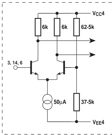
Fig. 8b F1/F2 data and power down inputs
