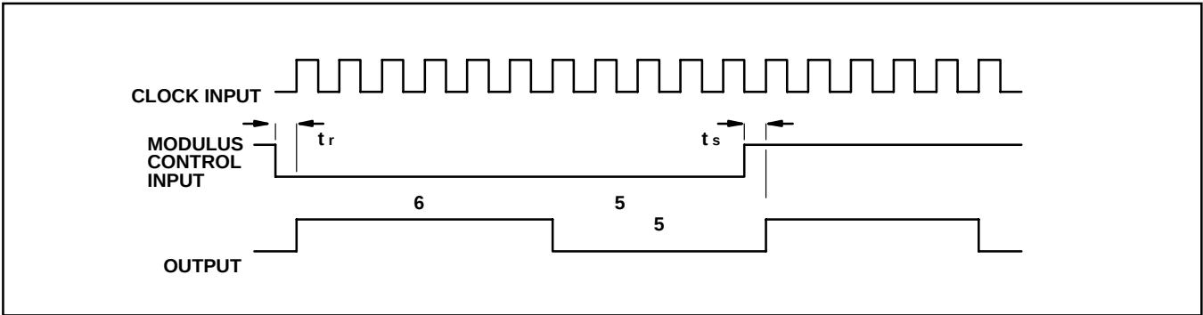
Fig.4 Timing diagram
