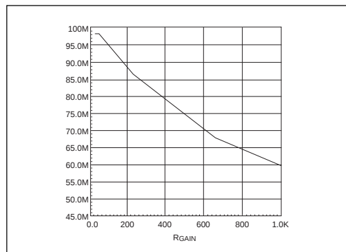
Figure 3. System Bandwidth versus Gain Resistor, V_{CC} = 5V , T = 27C .
