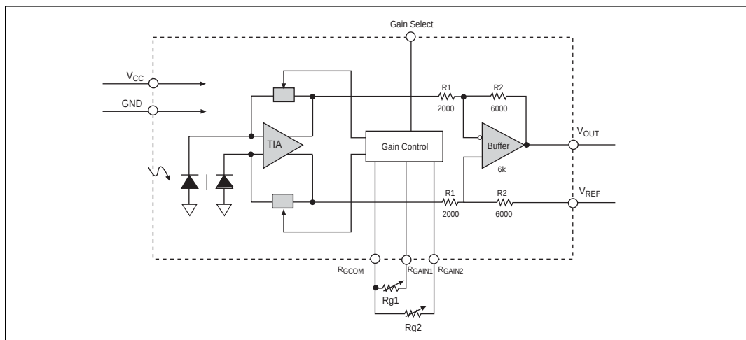
Figure 1. Functional Diagram
