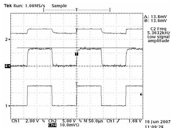
PWM 50% Duty Cycle Single LED 5kHz
