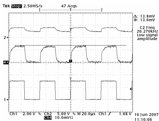
PWM 50% Duty Cycle Single LED 20kHz
