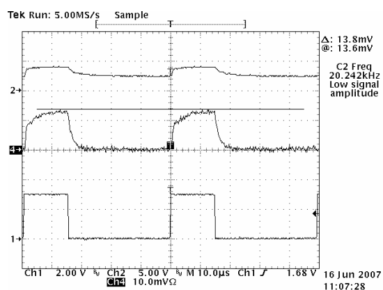
PWM Minimum Duty Cycle 15uS Single LED 20kHz
