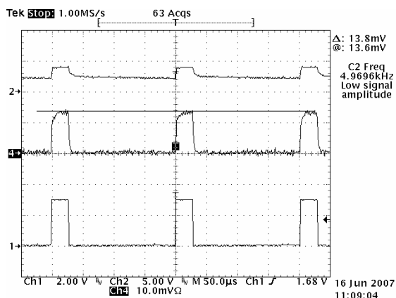
PWM Low Duty Cycle Single LED 5kHz
