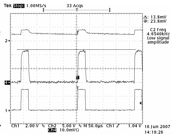
PWM Low Duty Cycle Single LED 5kHz
