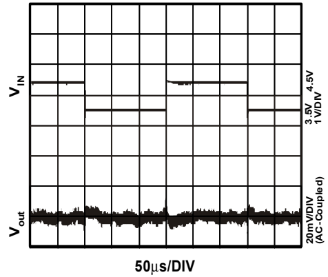
Line Transient
