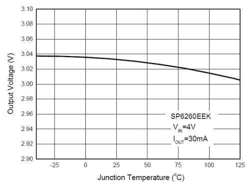
Fig. 14: Output Voltage vs. Junction Temperature SP6260EEK-L (3.0V)
