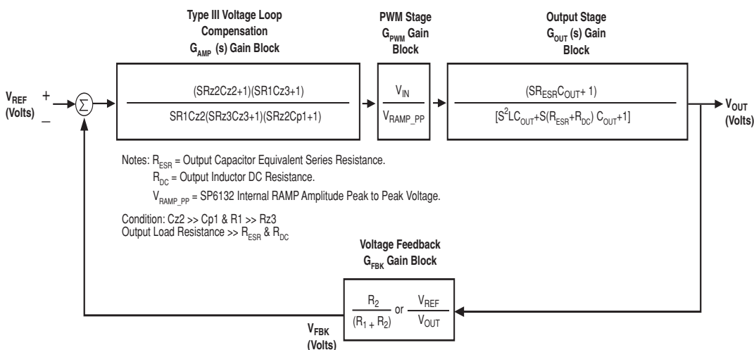
Figure 5: SP6138 Voltage Mode Control Loop with Loop Dynamic
