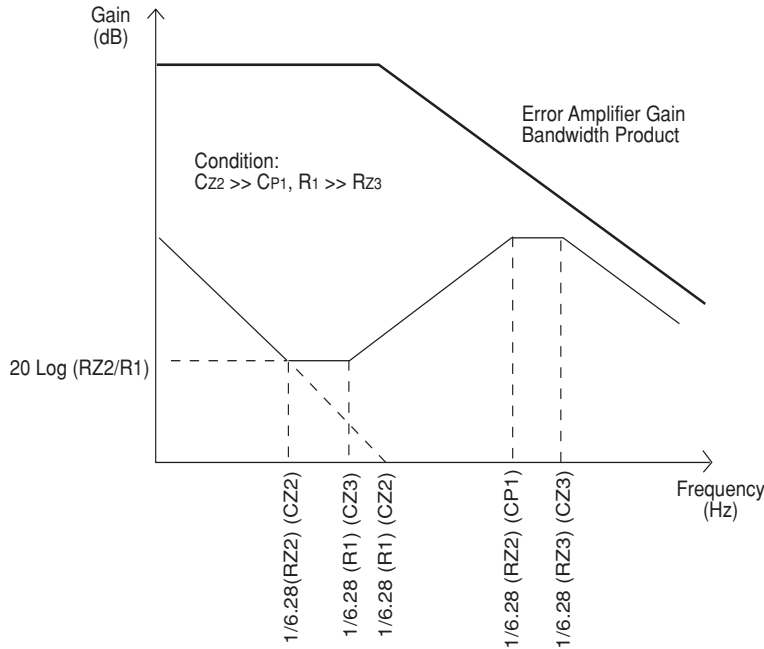
Figure 6: Bode Plot of Type III Error Amplify Compensation
