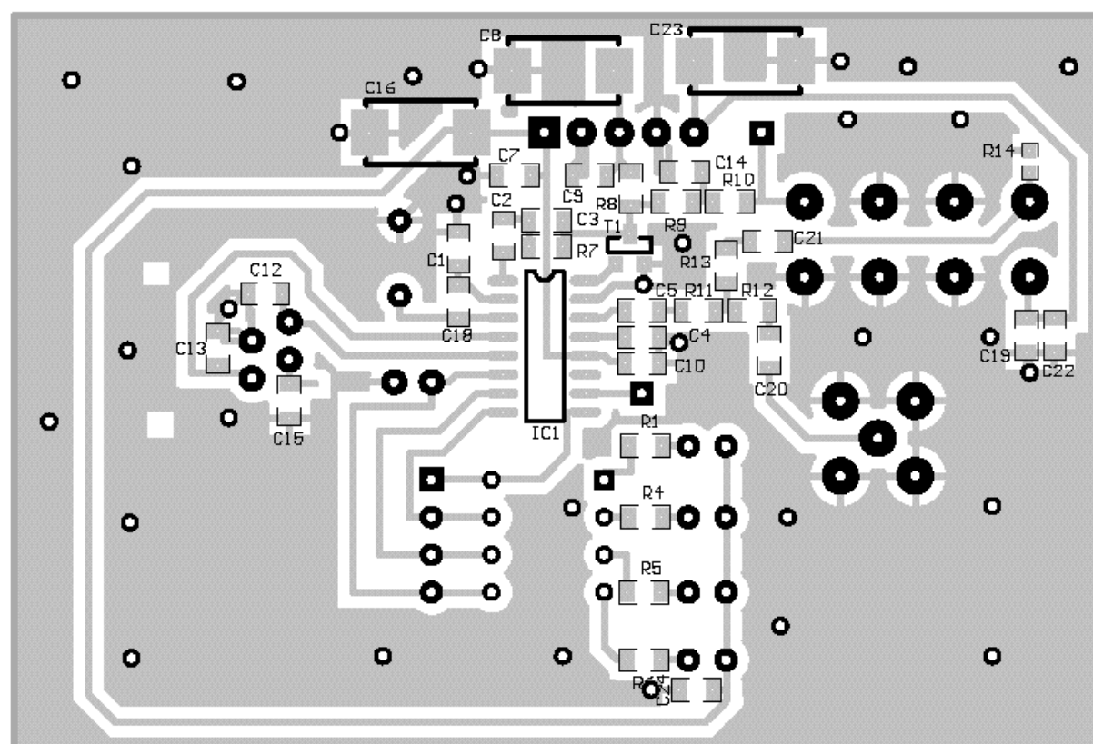
Bottom view
