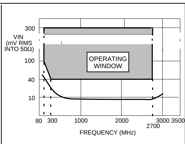
Fig. 5b Typical input sensitivity (Prescaler enabled, PE=1)
