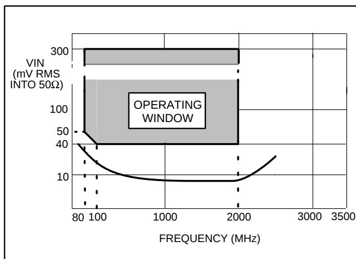
Fig. 5a Typical input sensitivity (Prescaler disabled, PE=0)
