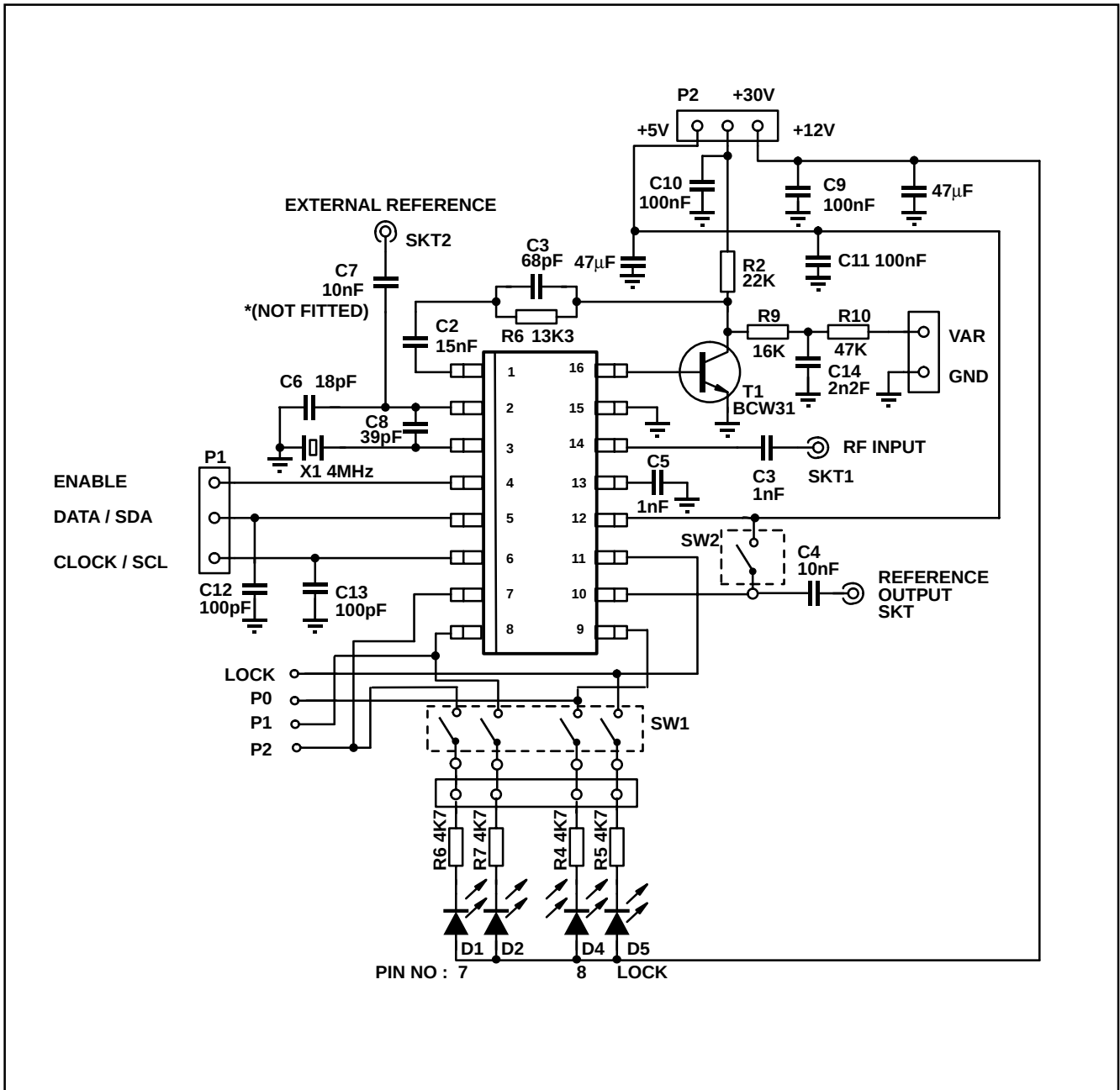
Fig. 8 Evaluation board
