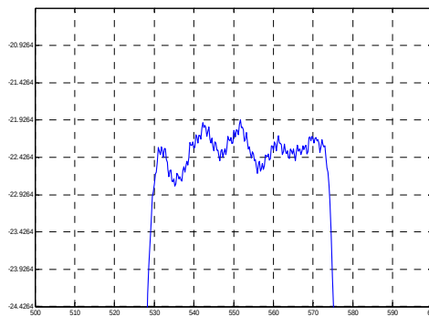
Passband Response
