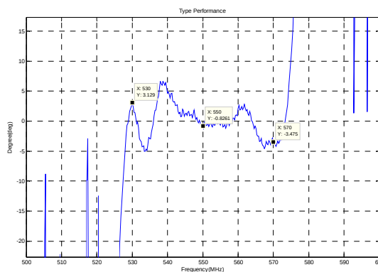
Phase Linearity(f0±20MHz)
