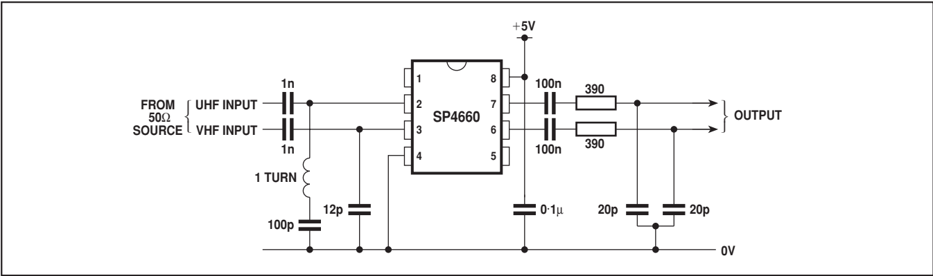
Fig. 4 Application circuit
