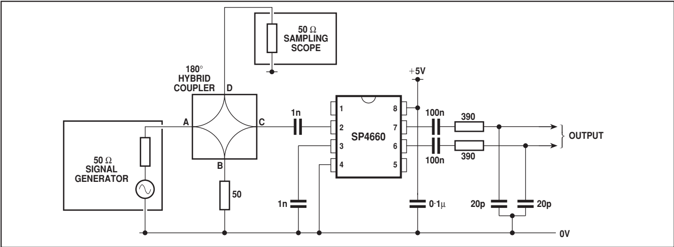
Fig. 3 Test circuit
