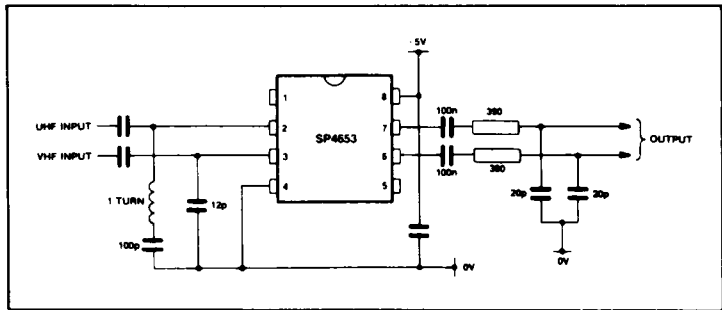
Fig.4 Application circuit
