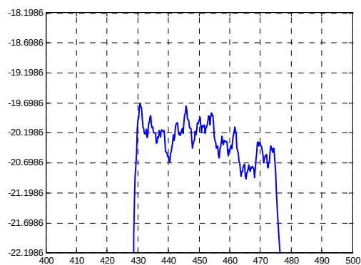
Passband Response
