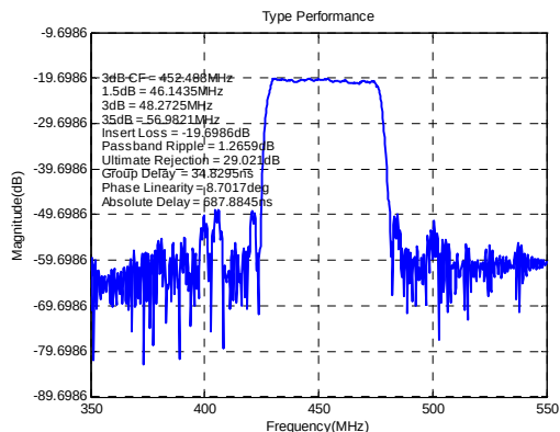
Frequency Response
