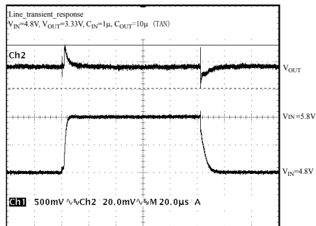
Figure 14. Line Transient Response
