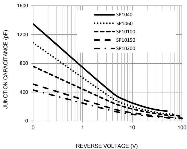
FIG. 5-TYPICAL JUNCTION CAPACITANCE
