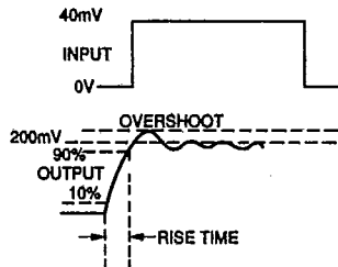
Transient Response
