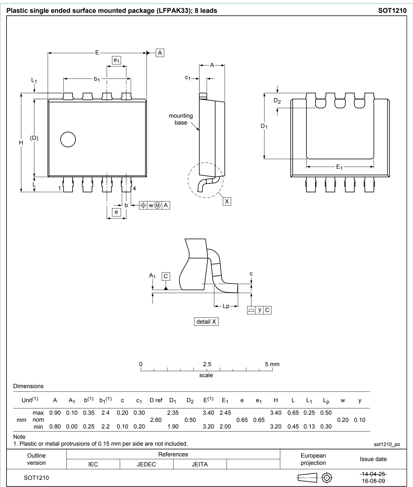
Fig. 1. Package outline LFAK33 (SOT1210)
