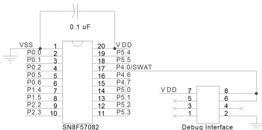
example circuit
