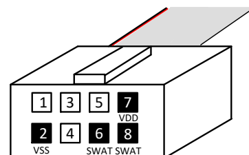
SN-Link header
