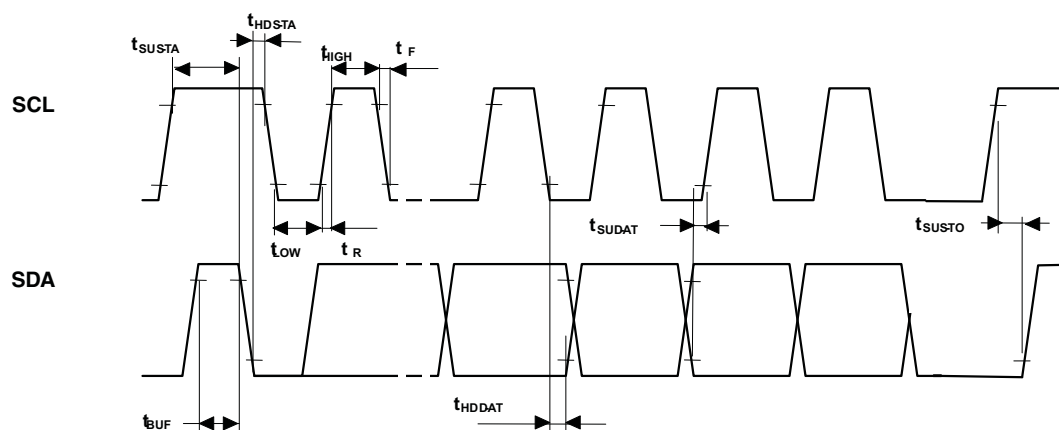
Figure 24. I²C Timing Chart
