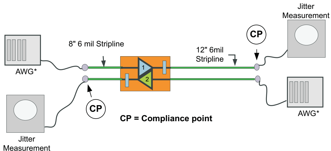
Figure 9. Jitter Measurement Test Condition
