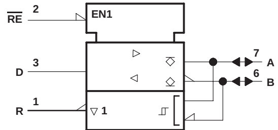
logic symbol†
