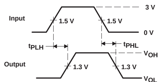
VOLTAGE WAVEFORMS
